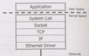
Figure 1: In a traditional network stack, applications interface with the network through a set of system calls (e.g., socket , bind , send ), and all network processing is performed in the kernel.
