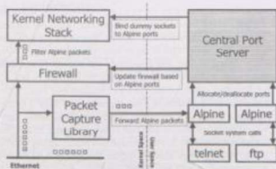
Figure 3: The role of Alpine's central port server is shown. The central server is responsible for allocating ports to each Alpine process. It uses a dummy socket to prevent the kernel from binding another socket to the port, and it uses a firewall to prevent the kernel's stack from reacting to packets sent to the bound port.
