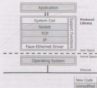
Figure 2: In Alpine the unmodified networking code is placed in a user-level library. An application is not modified because it interfaces with the library using the traditional socket system API.
