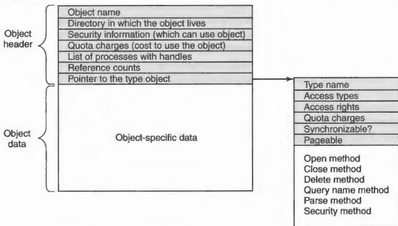
Figure 11-9. The structure of an object.
