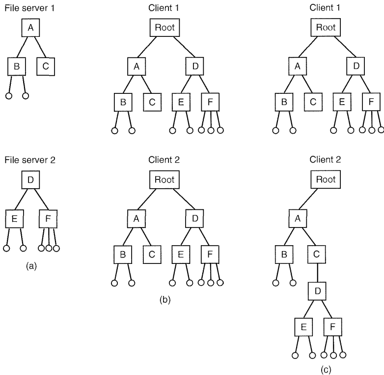
Figure 8-35. (a) Two file servers. The squares are directories and the circles are files. (b) A system in which all clients have the same view of the file system. (c) A system in which different clients may have different views of the file system.
