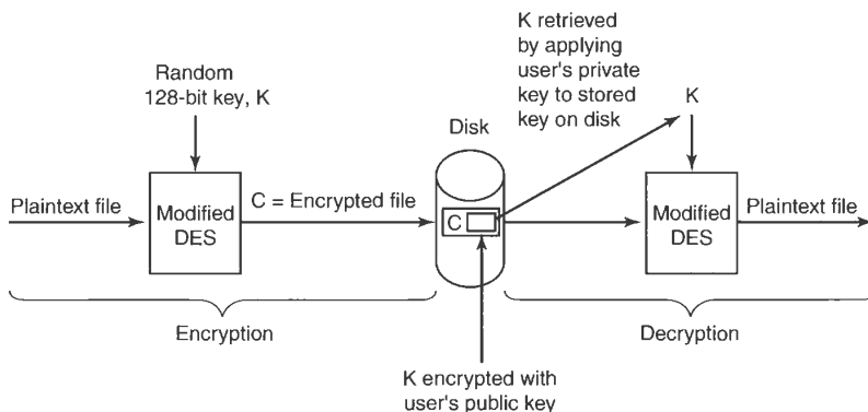
Figure 11-41. Operating of the encrypting file system.
