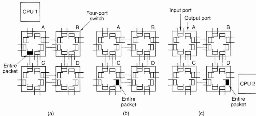
Figure 8-17. Store-and-forward packet switching.
