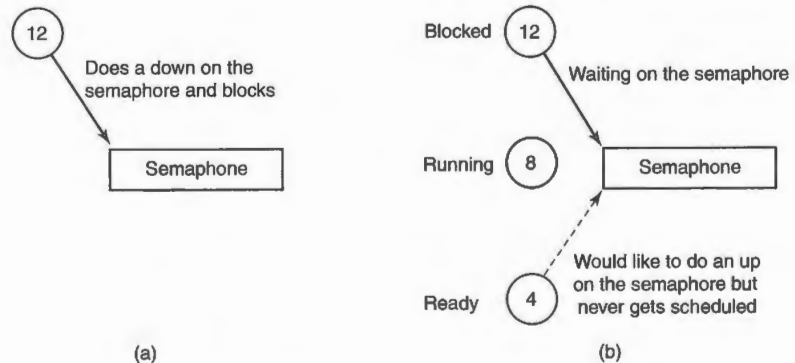
Figure 11-20. An example of priority inversion.
