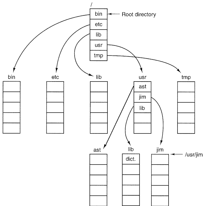
Figure 6-10. A UNIX directory tree.
