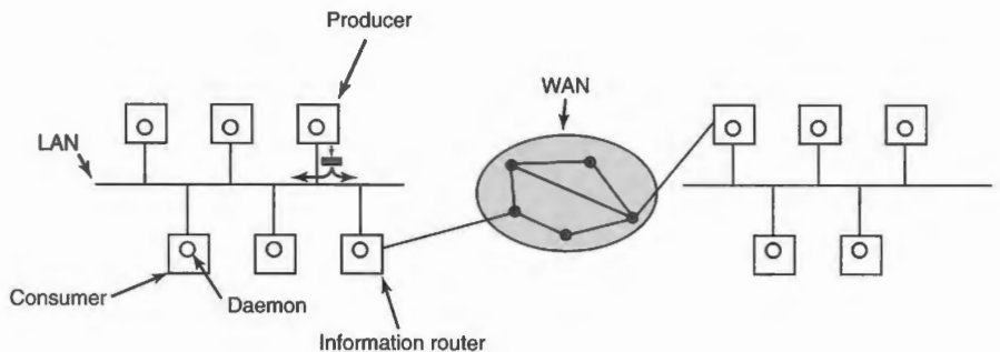
Figure 8-43. The publish/subscribe architecture.
