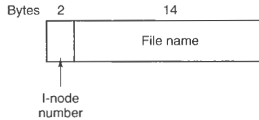
Figure 6-37. A UNIX V7 directory entry.
