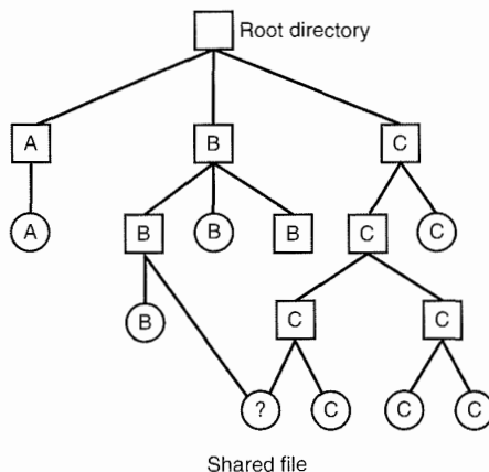
Figure 6-18. File system containing a shared file.
