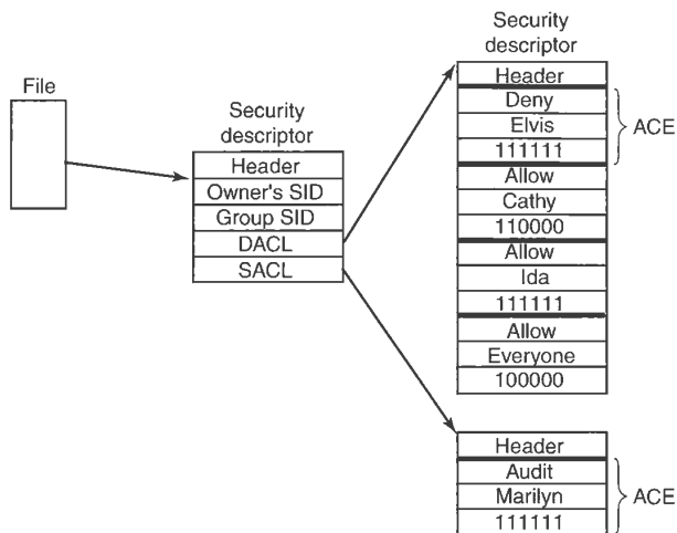
Figure 11-43. An example security descriptor for a file.
