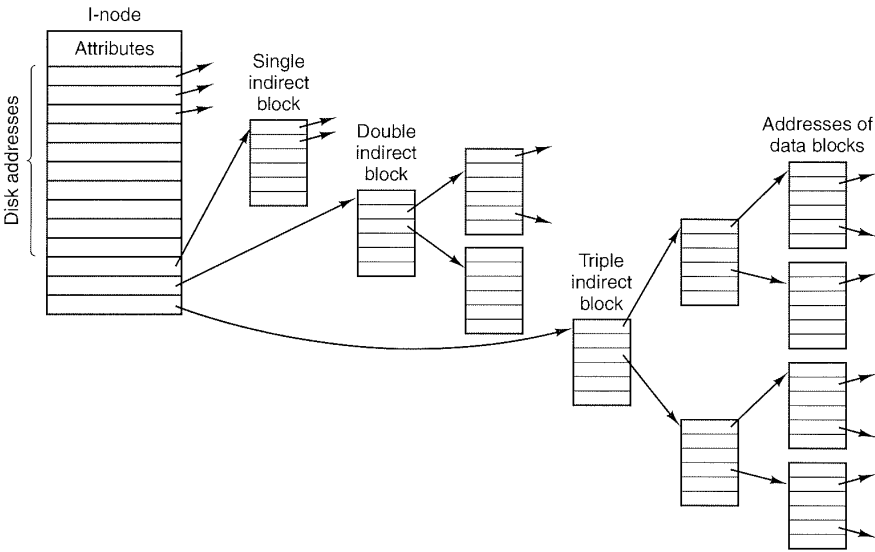
Figure 6-38. A UNIX i-node.
