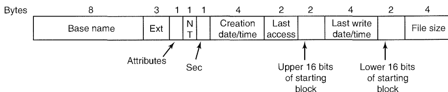
Figure 6-34. The extended MOS-DOS directory entry used in Windows 98.
