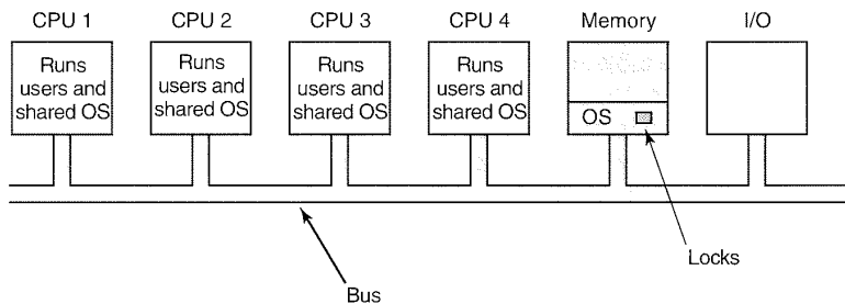
Figure 8-9. The SMP multiprocessor model.
