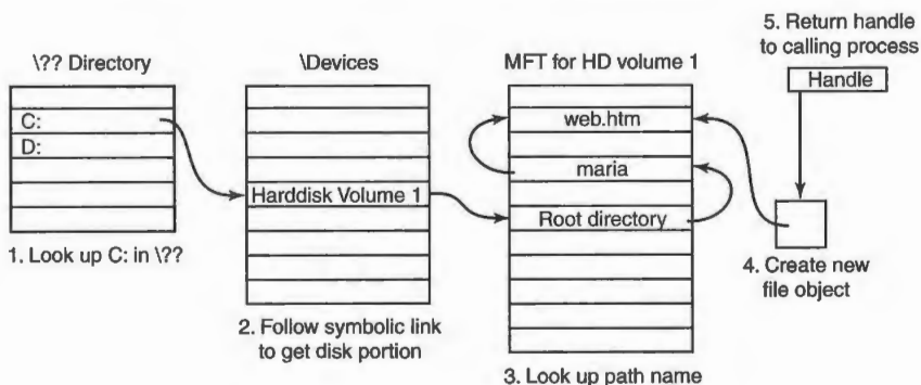
Figure 11-39. Steps in looking up the file C:\\maria\\web.htm .
