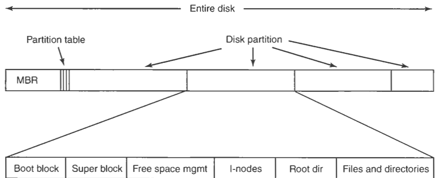
Figure 6-11. A possible file system layout.
