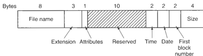
Figure 6-32. The MS-DOS directory entry.
