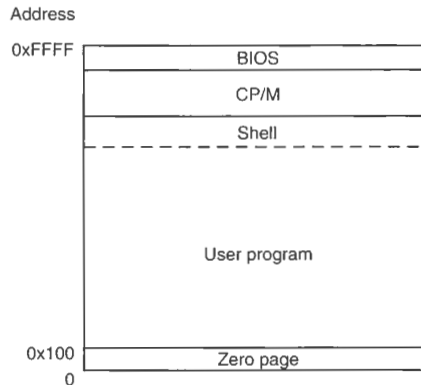
Figure 6-30. Memory layout of CP/M.
