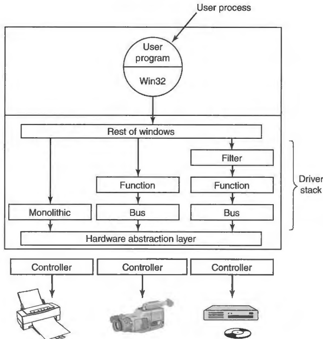
Figure 11-30. Windows 2000 allows drivers to be stacked.
