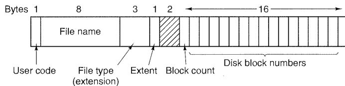
Figure 6-31. The CP/M directory entry format.
