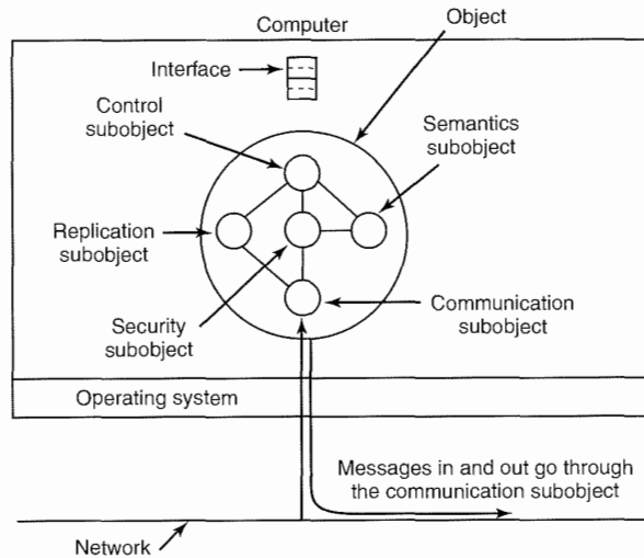
Figure 8-41. Structure of a Globe object.
