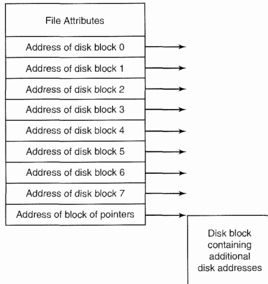
Figure 6-15. An example i-node.
