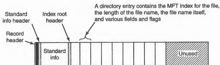
Figure 11-38. The MFT record for a small directory.
