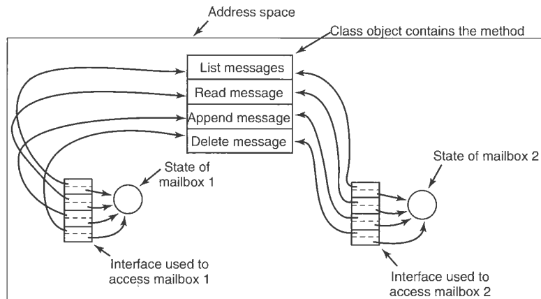
Figure 8-39. The structure of a Globe object.
