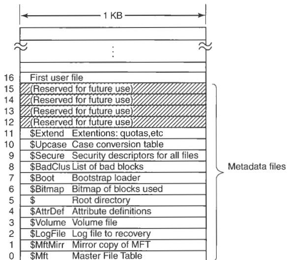
Figure 11-34. The NTFS master file table.
