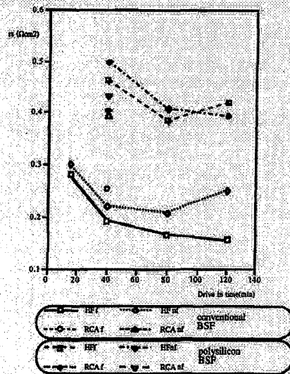
Fig.4 Total measured specific series resistance ( \Omega\text{cm}^2 ), in conventional and polysilicon BSF cells.
