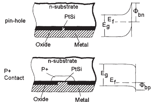
Figure 3. Back contact of rear PERL cell using PtSi film. Simplified energy band diagram illustrating the different contact barrier height at pin-hole and p + contact. At room temperature, PtSi/p-silicon contact (low barrier) presents a good ohmic characteristic.
