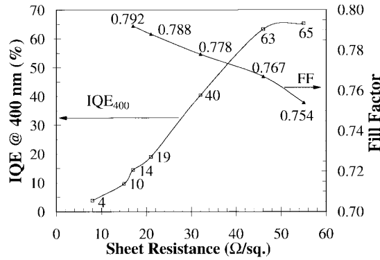
Fig. 2. Competition between enhanced short wavelength response and degraded FF with increasing \rho_s .
