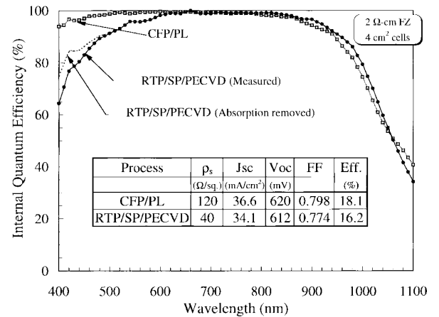
Fig. 3. Comparison of CFP/PL and RTP/SP/PECVD cells.
