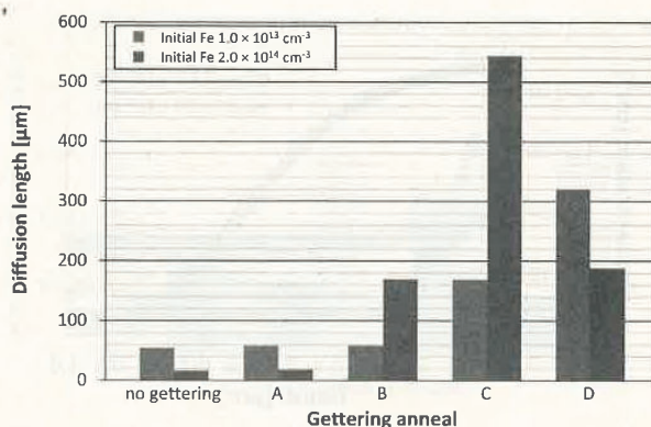
Fig. 2. Measured minority carrier diffusion length prior to dissociating the \text{Fe}_\text{B} -pairs in the same samples as in Fig. 1.
