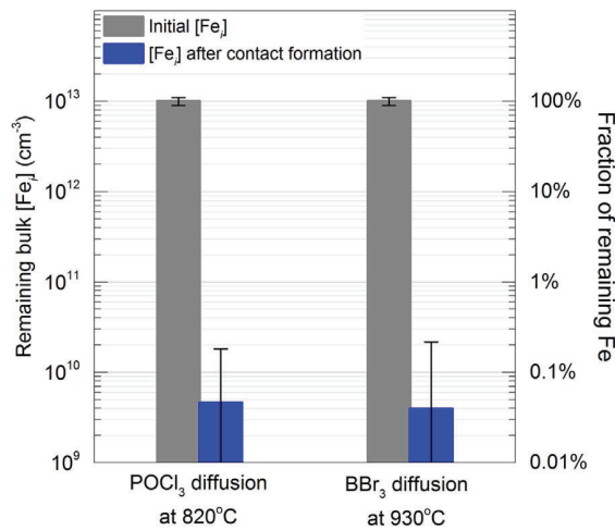
Fig. 2. Bulk interstitial Fe concentrations in silicon wafers before and after the formation of diffusion-doped polysilicon/oxide passivating contacts. The process parameters used for these two samples give the optimum passivating contact properties (optimum combination of surface passivation and contact conductivity).
