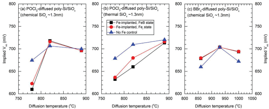
Fig. 4. Measurements of the 1-sun implied open circuit voltage ( iV_{oc} ) for samples with and without initial bulk Fe_i concentrations of 10^{13}cm^{-3} , that underwent the formation of (a) phosphorus-diffused polysilicon with \sim 1.3 nm chemical oxide interlayer; (b) phosphorus-diffused polysilicon with \sim 1.3 nm thermal oxide interlayer; (c) boron-diffused polysilicon with \sim 1.3 nm chemical oxide interlayer. The measured iV_{oc} are plotted against diffusion temperatures.
