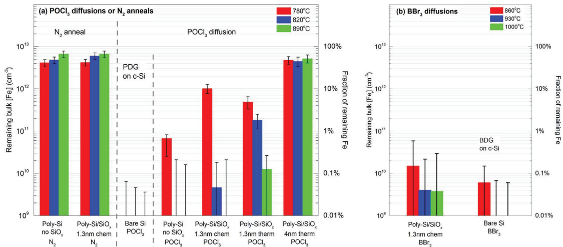
Fig. 3. (a) Comparison of the remaining bulk Fe i concentrations in samples with intrinsic polysilicon layers annealed in N 2 (with and without chemical oxide interlayer); with POCl 3 diffusions performed on bare crystalline silicon (c-Si) wafers, i.e. conventional phosphorus diffusion gettering (PDG); and with POCl 3 -diffused polysilicon layers in the presence of different oxide interlayers (no oxide, chemical oxide of ~1.3 nm, thermal oxide of ~1.3 nm, and thermal oxide of ~4 nm). The N 2 anneal and POCl 3 diffusion temperatures are 780 °C, 820 °C, and 890 °C, and the temperature-time profiles are the same for each temperature. (b) Comparison of the remaining bulk Fe i concentrations in samples that underwent the same BBr 3 diffusions with and without the polysilicon/oxide layers (1.3 nm chemical oxide). The BBr 3 diffusion temperatures are 860 °C, 930 °C, and 1000 °C. All samples had an initial bulk Fe i concentration of 10 13 cm -3 .
