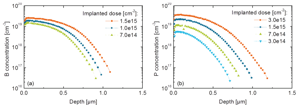
Fig. 2. ECV profiles measured on planar samples after ion implantation and annealing for 80 min at 1050 \text{ }^{\circ}\text{C} . (a) High dose boron implantations for the emitter; (b) phosphorus implantations for the back surface field.
