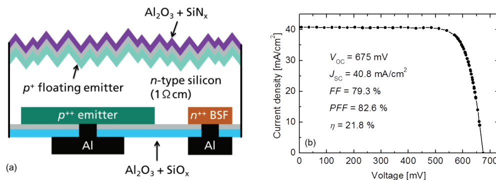
Fig. 3. (a) Cross-sectional sketch of the fabricated IBC solar cells; (b) IV data of the best cell measured in-house. Active cell area is 2 \times 2 \text{ mm}^2 , thickness is 200 \text{ } \mu\text{m} , pitch is 2.1 \text{ mm} .
