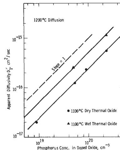
Fig. 3. Surface concentration dependence of phosphorus slow diffusivity in SiO_2 at 1200°C.
