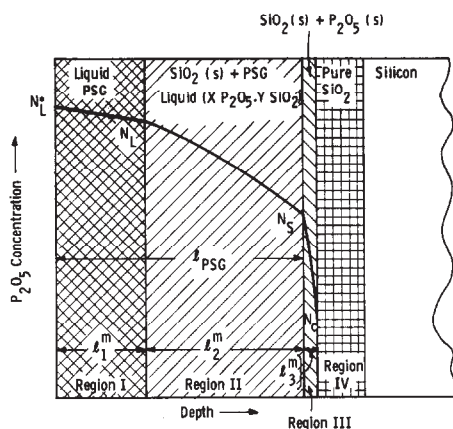
Fig. 4. Diagrammatic representation of the phosphosilicate glass structure on silicon. See text for explanation.
