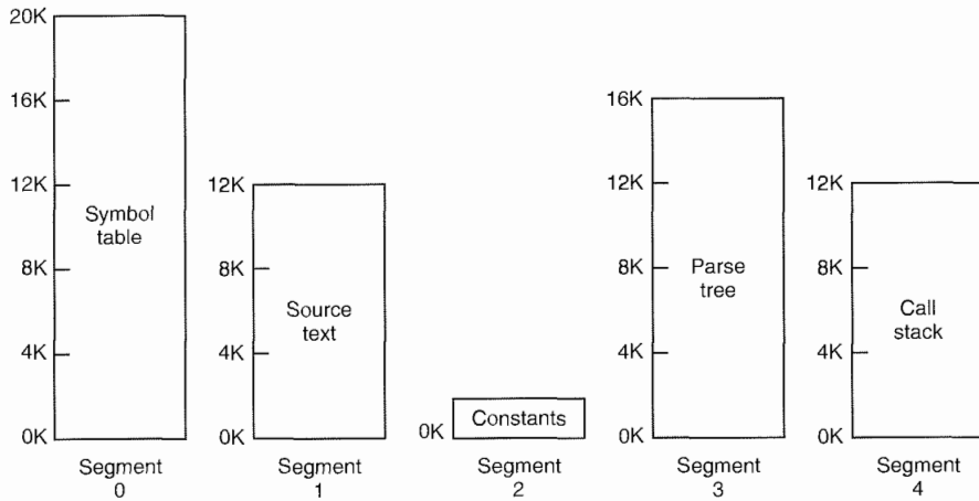
Figure 4-36. A segmented memory allows each table to grow or shrink independently of the other tables.
