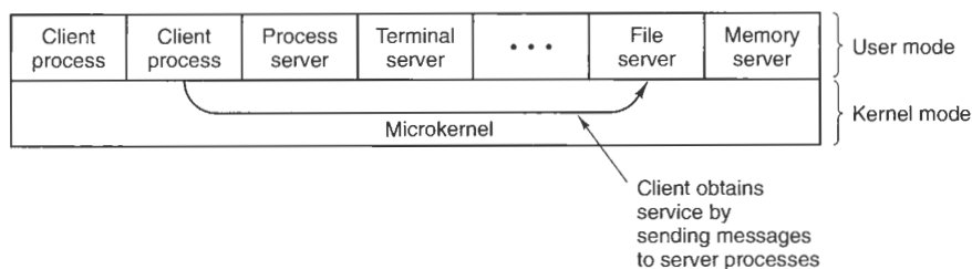
Figure 1-27. The client-server model.
