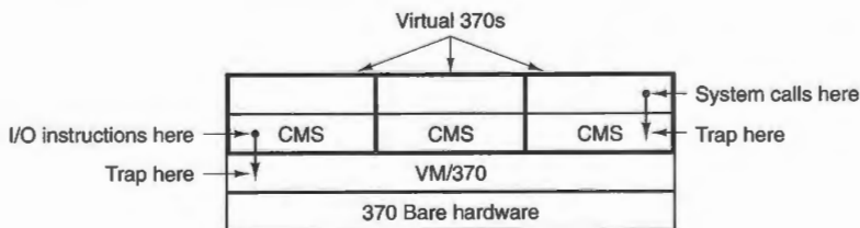
Figure 1-26. The structure of VM/370 with CMS.
