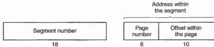
Figure 4-40. A 34-bit MULTICS virtual address.
