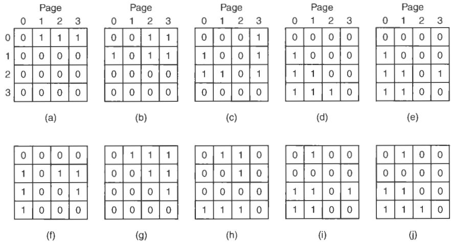
Figure 4-18. LRU using a matrix when pages are referenced in the order 0, 1, 2, 3, 2, 1, 0, 3, 2, 3.
