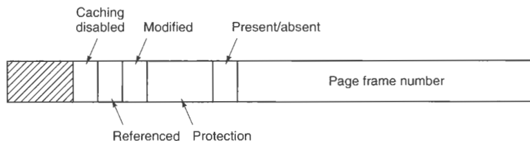
Figure 4-13. A typical page table entry.
