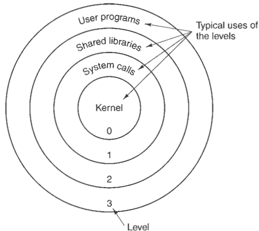
Figure 4-47. Protection on the Pentium.
