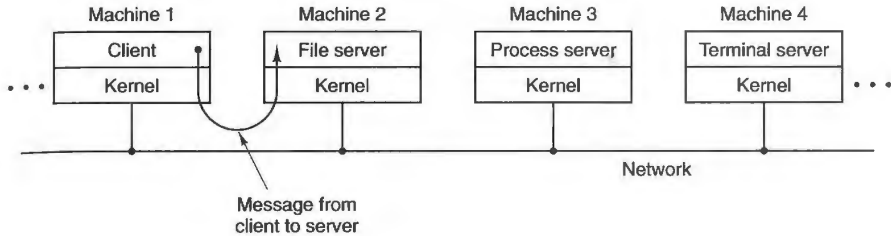
Figure 1-28. The client-server model in a distributed system.
