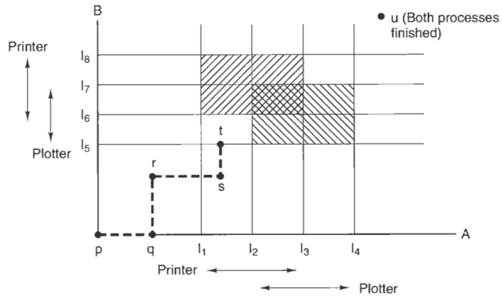
Figure 3-8. Two process resource trajectories.
