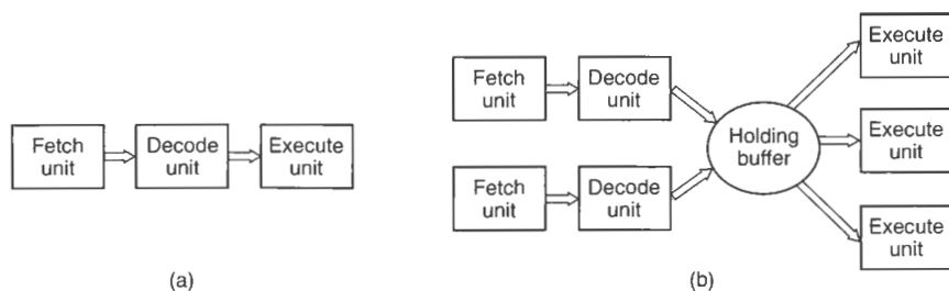
Figure 1-6. (a) A three-stage pipeline. (b) A superscalar CPU.
