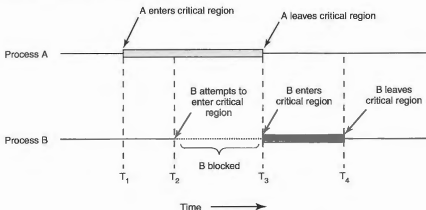
Figure 2-19. Mutual exclusion using critical regions.
