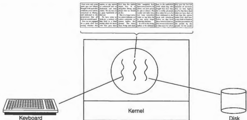
Figure 2-9. A word processor with three threads.
