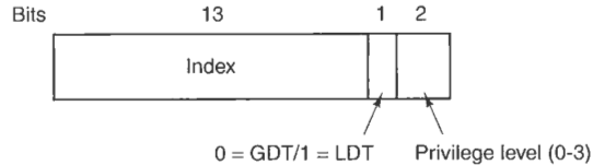
Figure 4-43. A Pentium selector.
