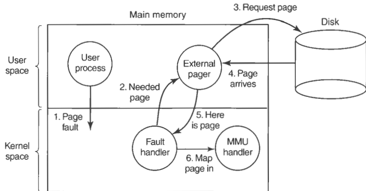
Figure 4-34. Page fault handling with an external pager.
