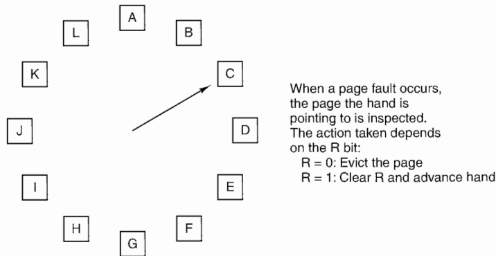
Figure 4-17. The clock page replacement algorithm.
