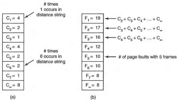
Figure 4-27. Computation of the page fault rate from the distance string. (a) The C vector. (b) F vector.
