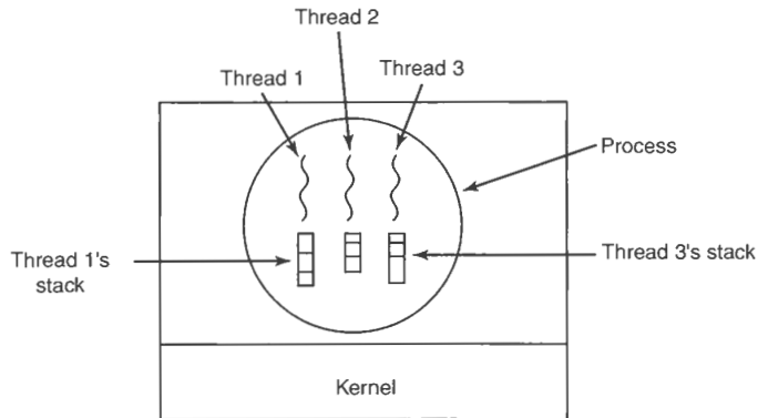
Figure 2-8. Each thread has its own stack.
