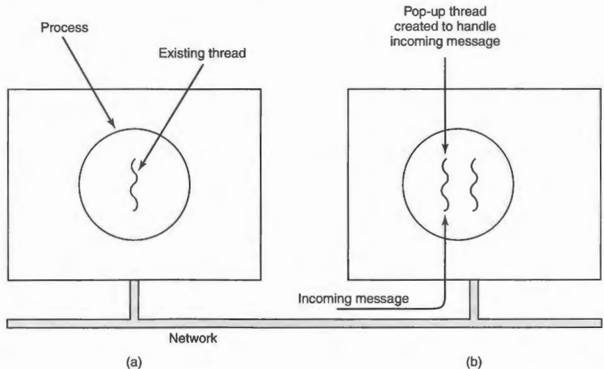
Figure 2-15. Creation of a new thread when a message arrives. (a) Before the message arrives. (b) After the message arrives.
