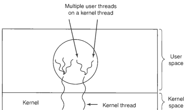
Figure 2-14. Multiplexing user-level threads onto kernel-level threads.
