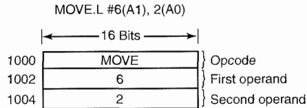
Figure 4-32. An instruction causing a page fault.
