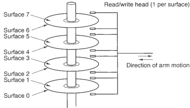
Figure 1-8. Structure of a disk drive.
