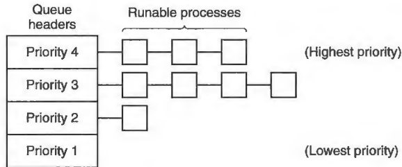
Figure 2-42. A scheduling algorithm with four priority classes.
