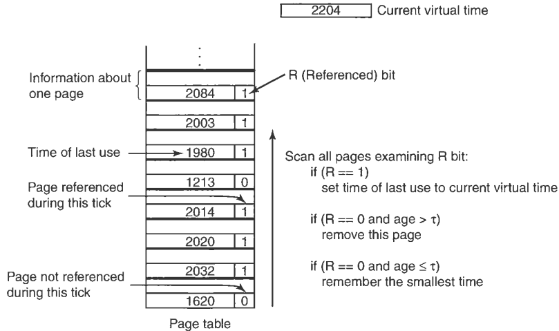
Figure 4-21. The working set algorithm.
