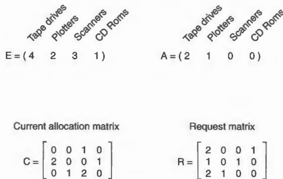
Figure 3-7. An example for the deadlock detection algorithm.
