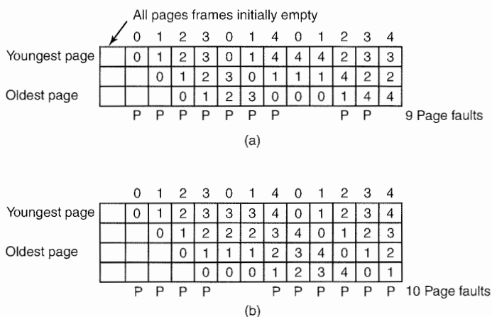
Figure 4-24. Belady's anomaly. (a) FIFO with three page frames. (b) FIFO with four page frames. The P's show which page references cause page faults.
