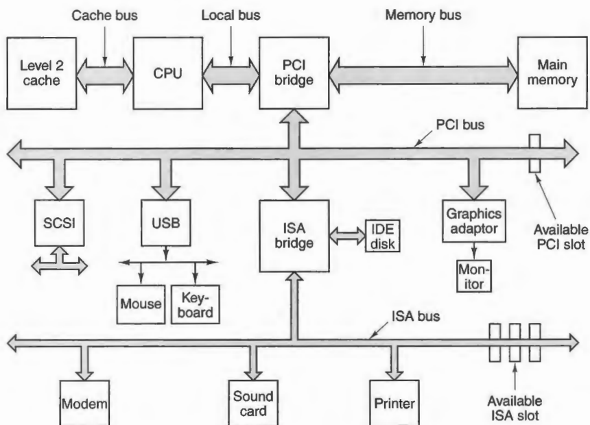
Figure 1-11. The structure of a large Pentium system
