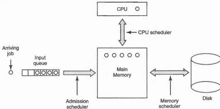
Figure 2-40. Three-level scheduling.
