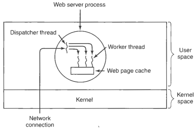
Figure 2-10. A multithreaded Web server.
