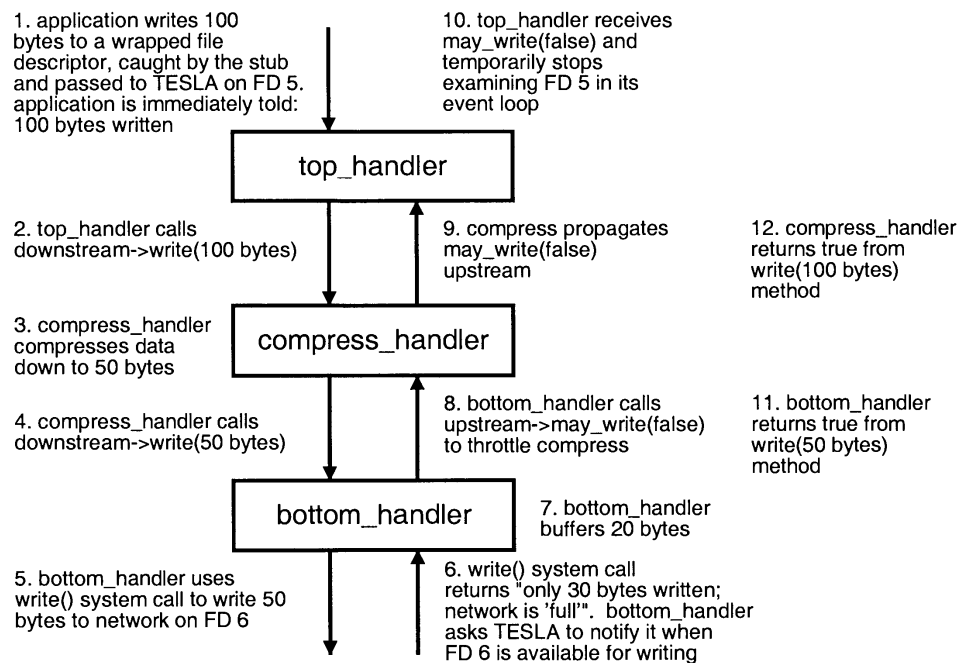
Figure 4-2: An application writes to a network flow which cannot presently deliver all the bytes via the underlying transport protocol (a TCP stream on file descriptor 6).
