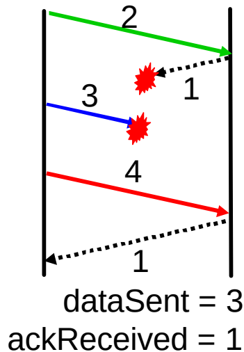
Figure 3.4: Example of basic loss deduction algorithm with fast ACK parity.
