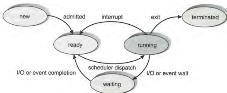
Figure 4.1 Diagram of process state.
