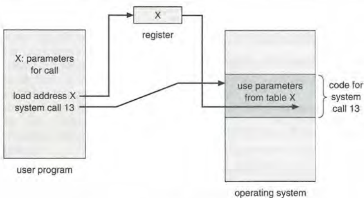
Figure 3.1 Passing of parameters as a table.
