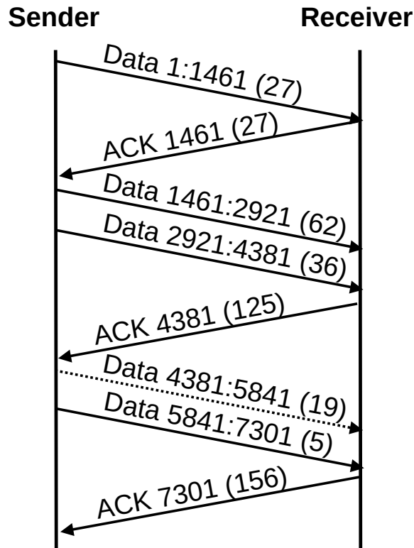
Figure 4.7: Time line for a data transfer using a cumulative nonce.
