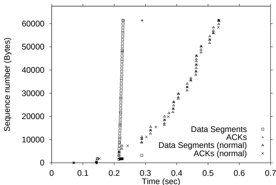
Figure 4.5: Time-sequence plot of TCP Daytona DupACK spoofing attack.
