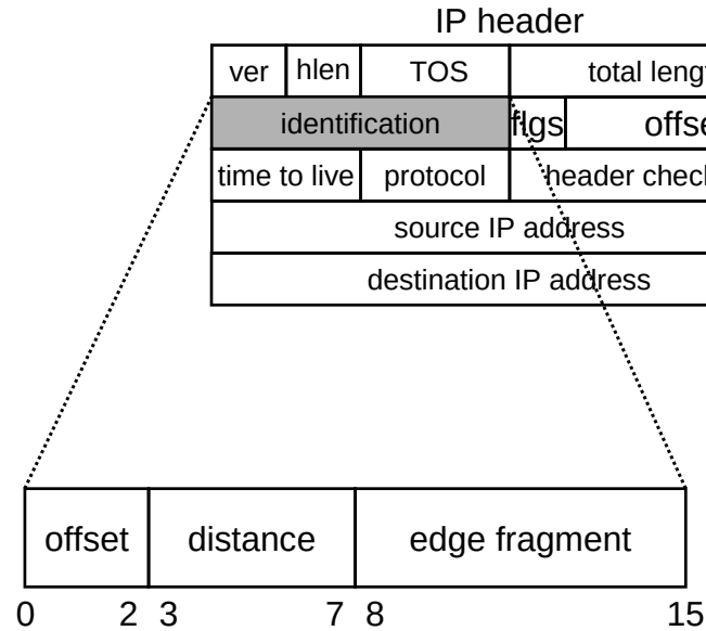
Figure 5.9: Encoding edge fragments into the IP identification field.
