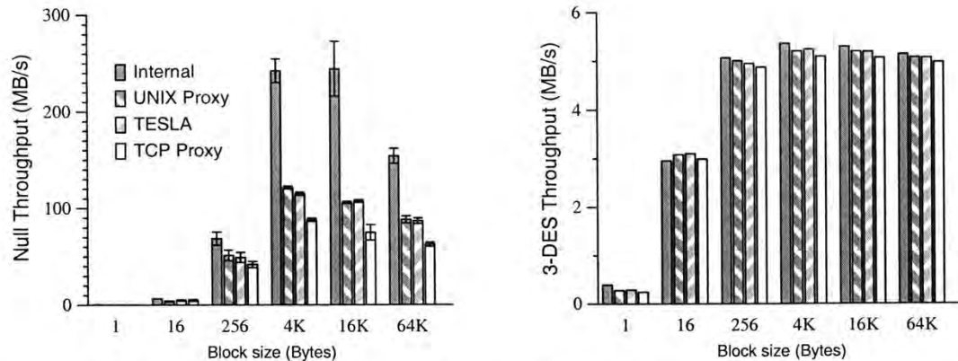
Figure 4-3: Results of the rbandwidth test. In the left graph, we show error bars at \pm 1 standard deviation; in the right graph, the variance was consistently very small. ( wbandwidth yielded results similar to rbandwidth .)
