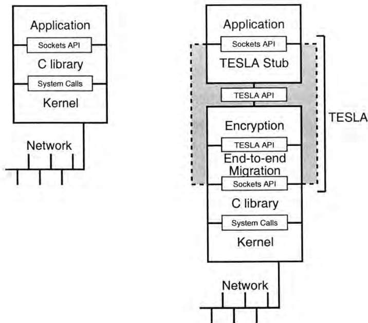
Figure 1-1: A typical networked system is at left. At right, we show a TESLA-enabled system with encryption and flow migration handlers enabled.
