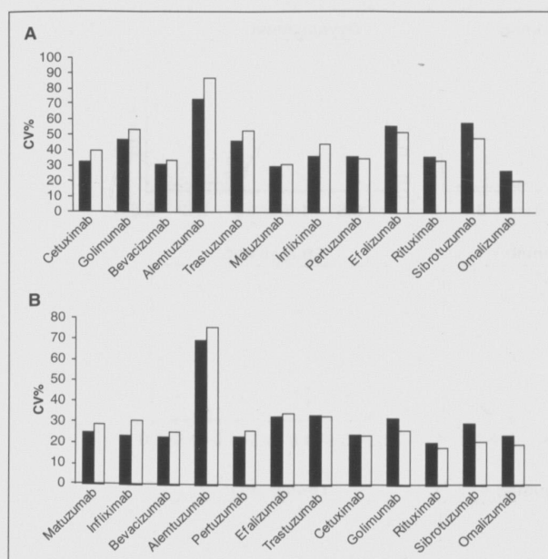
Figure 5. Comparison of the variability of simulated AUC (A) and Cmax (B) of 1000 subjects after receiving a single fixed (solid bar) and body weight/body surface area (BW/BSA)-based dose (open bar).
