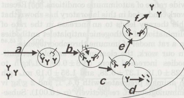
Figure 4. Proposed mechanism for IgG protection by FcRn. (a) IgG molecules enter cells (e.g., vascular endothelial cells, muscle cells, etc.) via pinocytosis (e.g., fluid-phase endocytosis); (b) H^+ enters the endosome, reducing pH, and IgG binds with FcRn; (c) the endosome fuses with the lysosome, but FcRn-bound IgG is not released to the lysosome; (d) unbound IgG is released to the lysosome and catabolized by proteases; (e) the endosome fuses with the plasma membrane, the FcRn–IgG complex is exposed to physiologic pH; and (f) IgG is released into plasma (or interstitial fluid).
