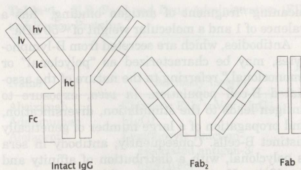
Figure 2. Structure of IgG and IgG fragments. Intact IgG is comprised of two heavy chains and two light chains. Heavy and light chains each contain a "constant" region (hc and lc) and a "variable" region (hv and lv). As noted in the text, the constant and variable regions allow consistency in antibody structure and diversity in antigen binding. The IgG molecule has a molecular weight of ~150 kDa and a valence of 2. The IgG fragments, Fab 2 and Fab, have molecular weights of ~110 and ~50 kDa, respectively.
