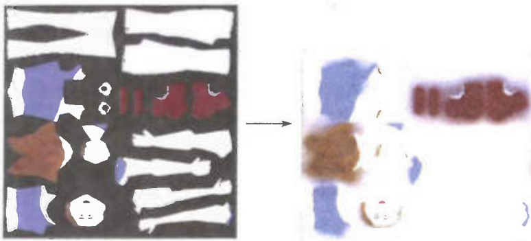
Figure 37-13. Color Extrapolation
