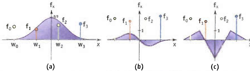
Figure 20-1. The Cubic B-Spline and Its Derivatives
