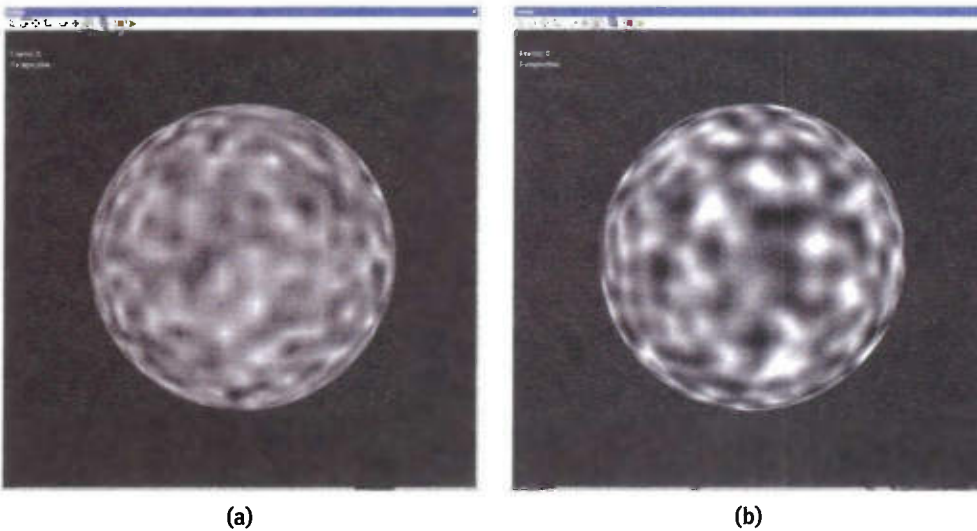
Figure 26-1. 3D Noise
