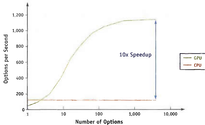
Figure 45-4. GPU vs. CPU Performance of a Binomial Lattice Model with N = 1024 Steps As with the Black-Scholes algorithm, the GPU implementation of the binomial method substantially outperforms the CPU implementation when more than a small number of pricing problems are solved in parallel. Unlike the Black-Scholes GPU implementation, I/O is not a substantial bottleneck in this case due to the large amount of computation performed for each result value.
