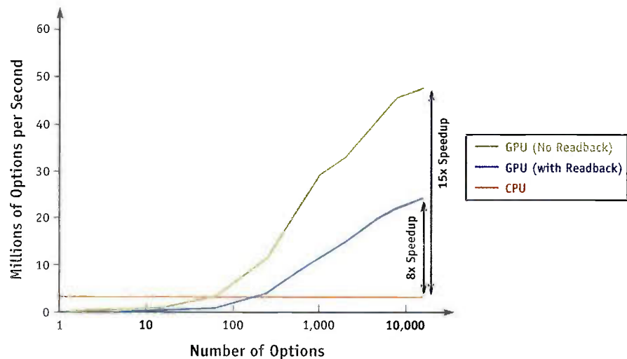
Figure 45-1. GPU vs. CPU Performance of Black-Scholes Option Pricing
