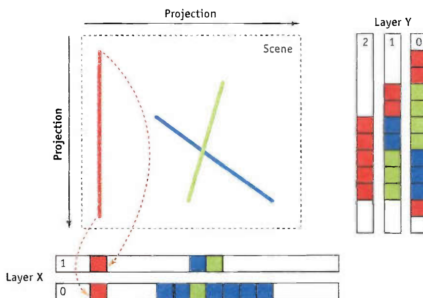
Figure 47-6. Voxelization Based on Depth Peeling
