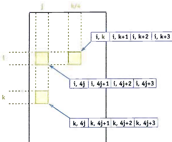
Figure 43-3. Data Packing for Vectorization
