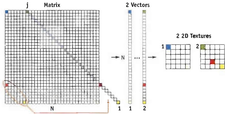
Figure 44-3. Representing a Banded Sparse Matrix on the GPU Two diagonals can be combined into one texture vector.
