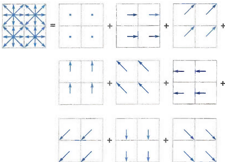
Figure 47-3. Division of a D2Q9 Model According to Its Velocity Directions A separate array is used for each velocity vector.
