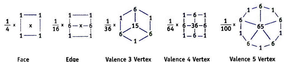
Figure 7-2. Catmull-Clark Subdivision Masks
