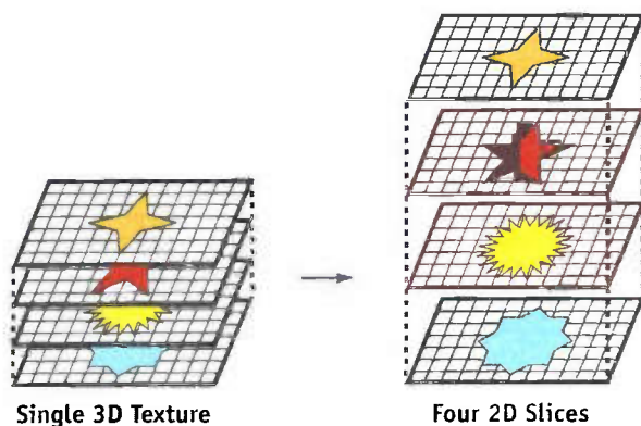
Figure 33-6. Storing a 3D Texture with Separate 2D Slices
