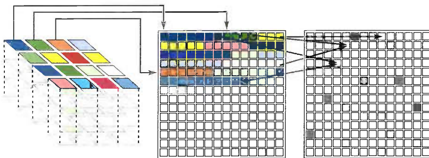
Figure 33-8. Purcell's Sparse Ray-Tracing Data Structure
