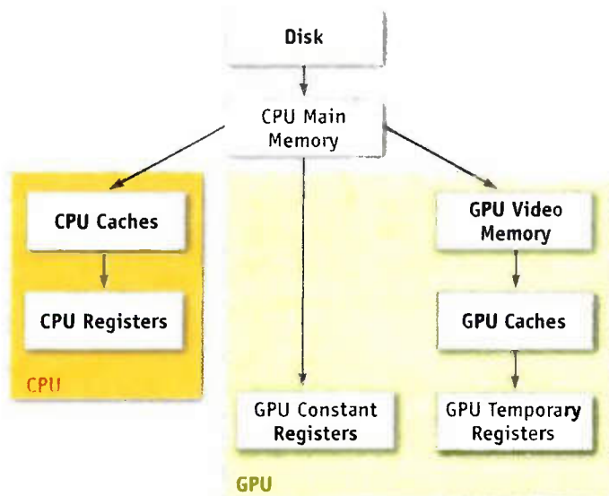
Figure 33-2. The CPU and GPU Memory Hierarchies
