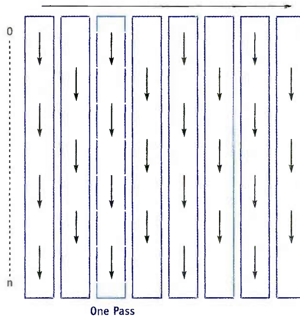
Figure 46-1. The Odd-Even Transition Sorting Network for n Keys Arrows indicate the compare operation "less-than".
