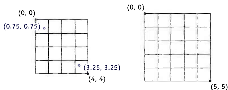
Figure 7-7. Resampling a Patch
