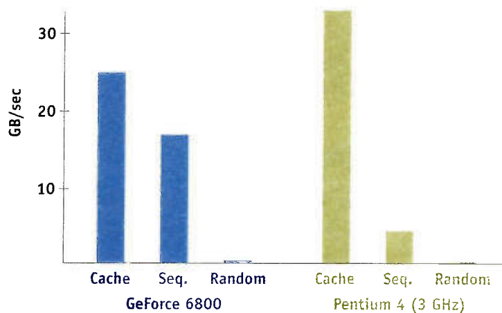
Figure 32-1. Comparing Memory Performance of the GPU and CPU
