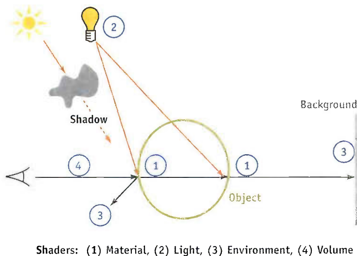
Figure 13-1. Shaders in a Scene
