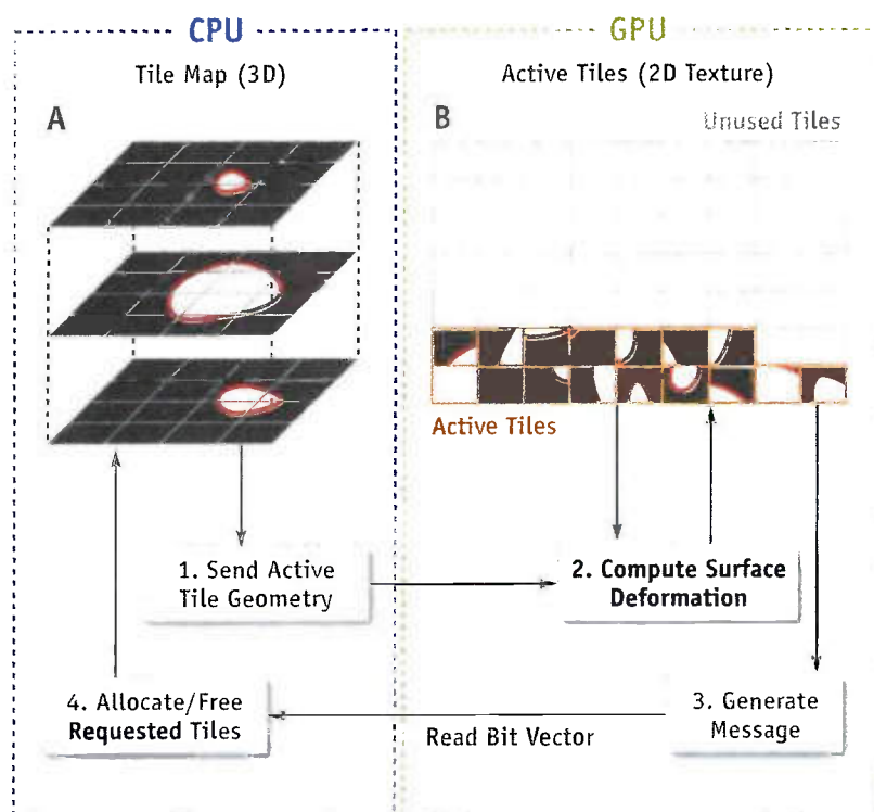
Figure 33-9. Dynamic Sparse Volume Data on the GPU
