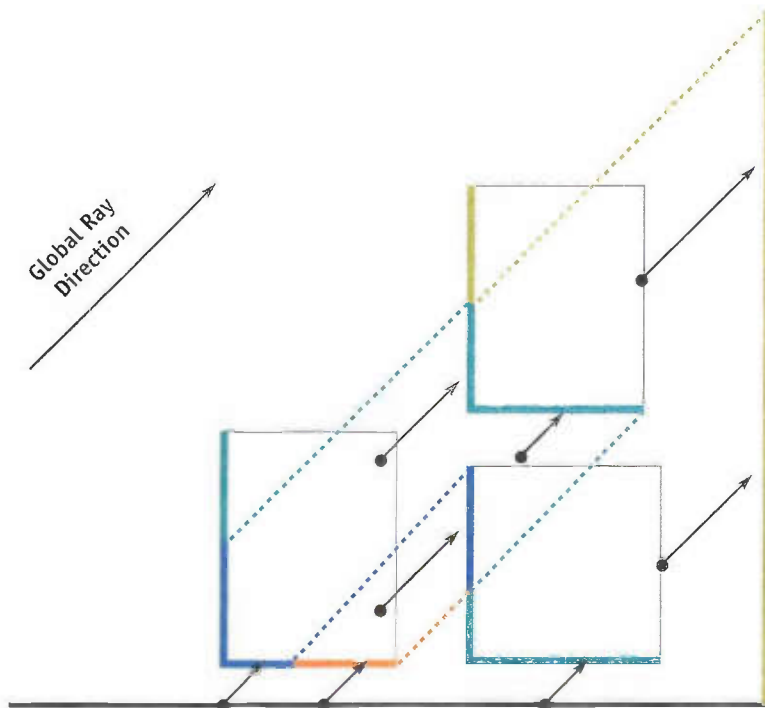
Figure 38-7. Parallel Multiple Ray Casts as a Parallel Projection
