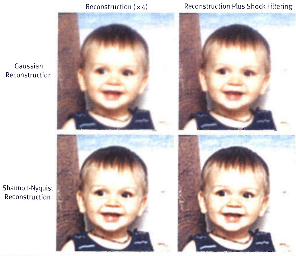
Figure 27-9. Shock Filtering
