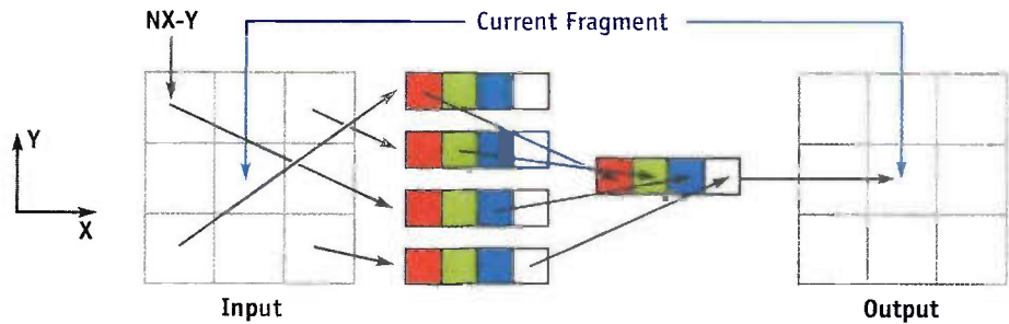
Figure 47-5. Streaming of Packet Distribution
