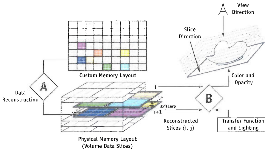
Figure 41-2. Rendering from a Custom Memory Format Using Deferred Filtering Step A shows reconstruction of a physical volume slice i + 1 . Step B renders trilinearly interpolated slices between i and i + 1 .
