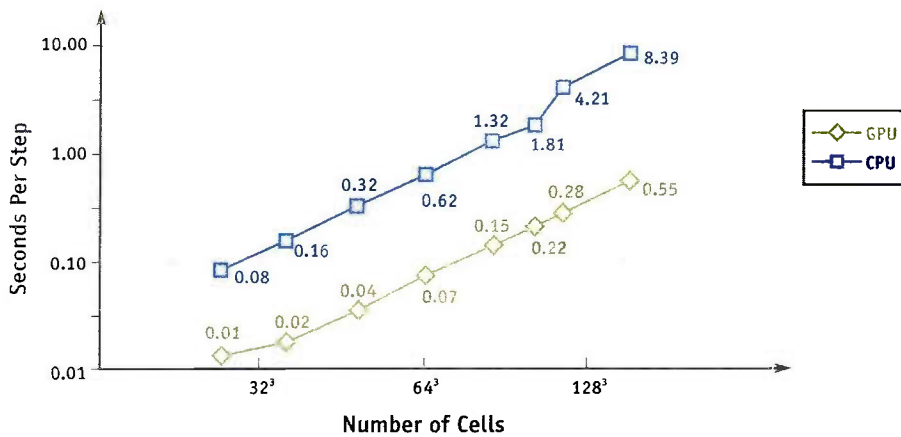
Figure 47-9. Time per Step of a D3Q19 LBM Simulation The GPU is typically 8 to 9 times faster, though it is 15 times faster for the 128^3 lattice.
