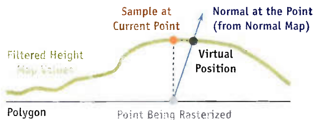
Figure 9-4. The Virtual Position Trick
