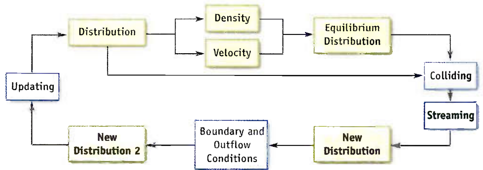
Figure 47-4. Flow Chart of LBM Computation on the GPU Green boxes are the textures, and blue boxes are operations.
