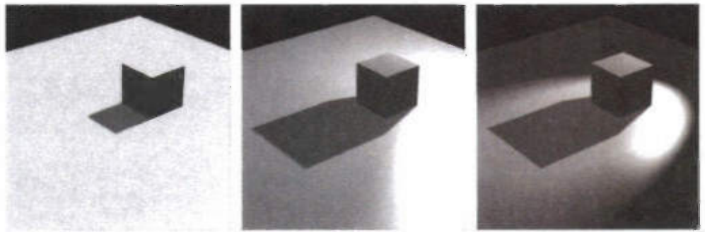
Figure 13-6. Directional, Point, and Spotlight Illumination and Shadow Map
