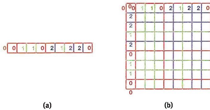
Figure 12-4. Examples of Tile Packing
