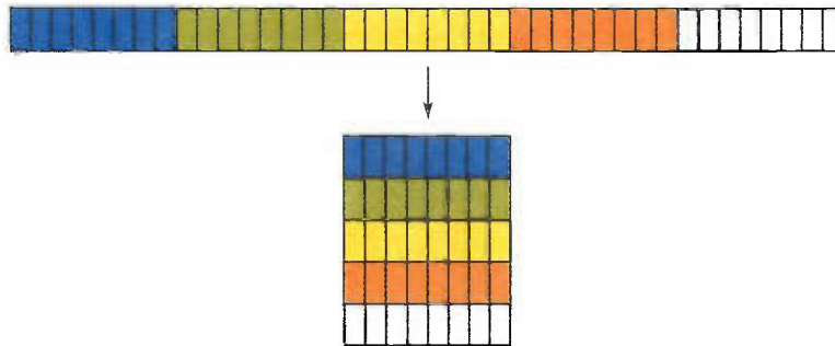
Figure 33-5. 1D Arrays Packed into 2D Arrays Doing so avoids the size restrictions that current GPUs place on 1D textures.
