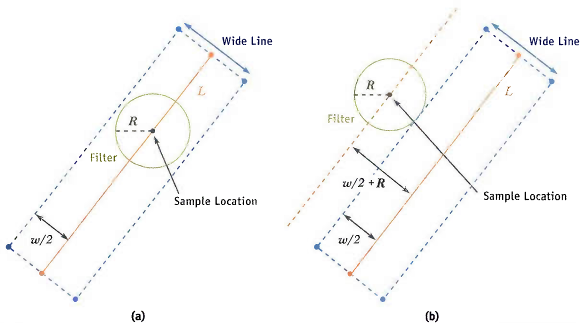
Figure 22-5. How Filter Placement Affects the Convolution (a) The value of the convolution is maximized when the filter is directly on L . (b) The value of the convolution is minimized when the filter is at a distance of w/2 + R from L .
