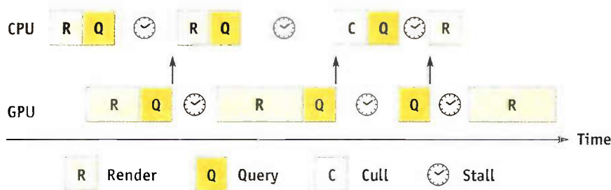
Figure 6-1. CPU Stalls and GPU Starvation Caused by Occlusion Queries
