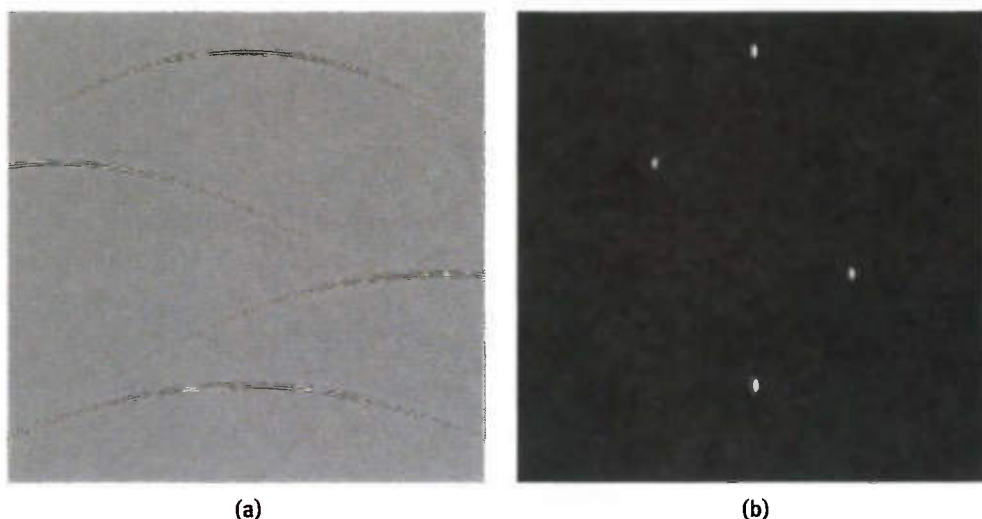
Figure 48-8. Simulated and Reconstructed Data of a Phantom (a) The simulated data of a phantom containing four pin targets. (b) The reconstructed data of the phantom.
