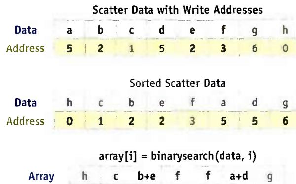
Figure 32-5. Converting Scatters to Gathers with Address Sorting
