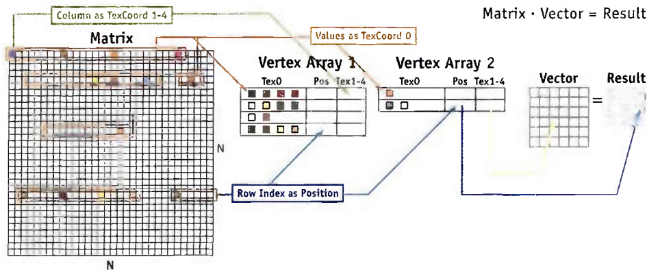
Figure 44-4. Representing a Random Sparse Matrix The matrix-vector product is explained in Section 44.3.3.
