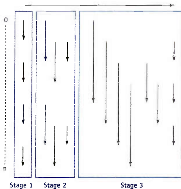
Figure 46-2. The Odd-Even Merge Sorting Network for n Keys Each stage establishes two partial sorts that are merged in the next stage.
