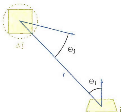
Figure 39-2. The Oriented-Disc Form Factor
