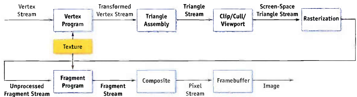
Figure 29-3. Mapping the Graphics Pipeline to the Stream Model
