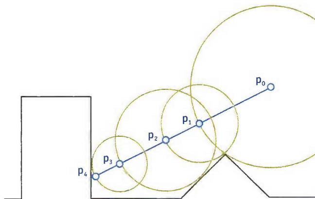
Figure 8-5. Sphere Tracing
