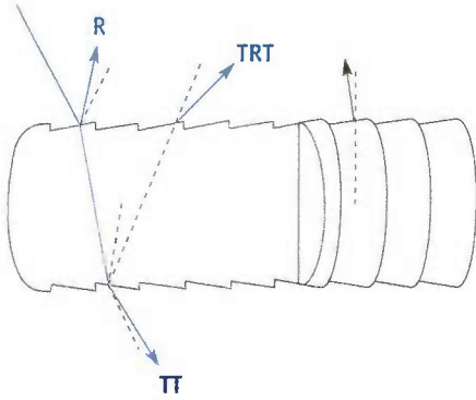
Figure 23-14. Reflectance Paths
