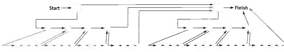
Figure 14-6. Hierarchical Elements
