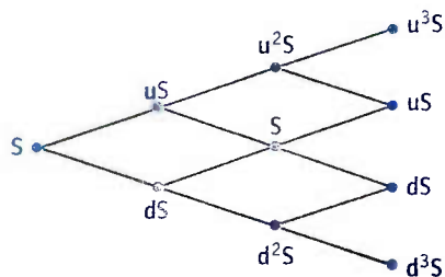
Figure 45-2. Binomial Tree of N = 3 Steps, with Associated Asset Prices
