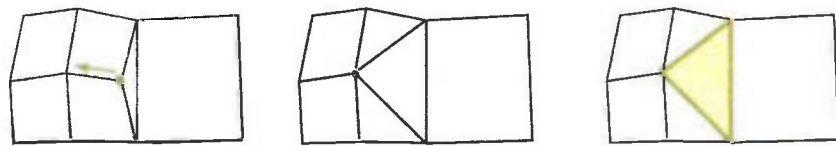
Figure 7-8. Handling T-Junctions
