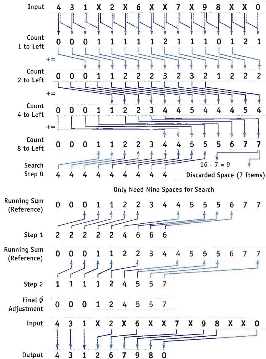
Figure 36-1. Iteratively Counting Null Records in a Stream At each iteration, each stream element sums the number of null elements at its position and progressive powers-of-two positions to the left. The end result lets a subsequent pass quickly determine how to compact the stream so that there are no null elements remaining.
