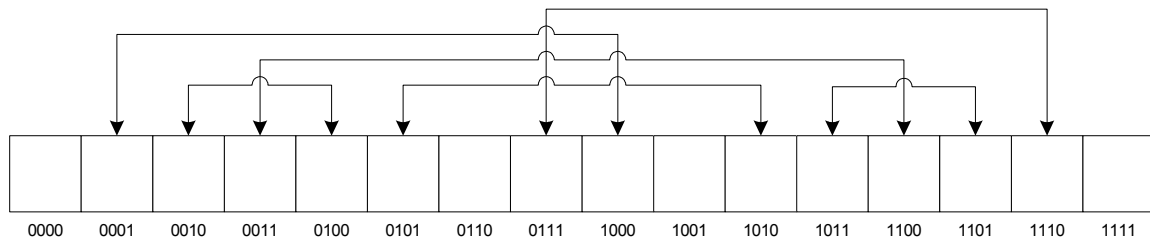
Figure 10 - Simple scramble of 16×1 image
