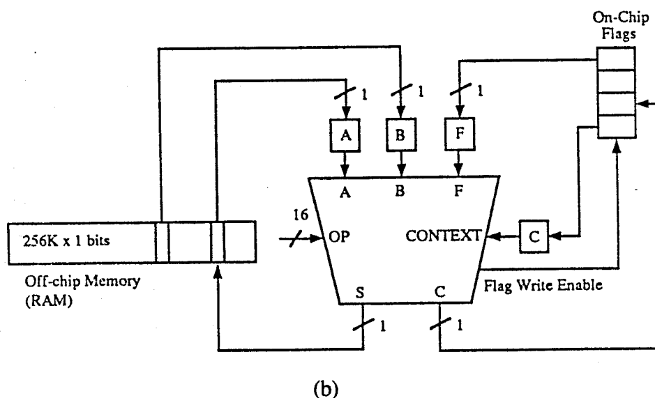
Examples of bit-serial PEs: a) LUCAS, b) Connection Machine
