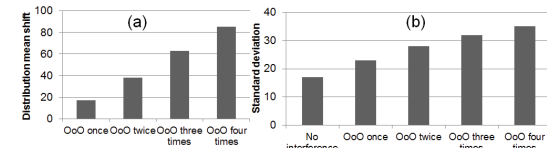
Fig. 7. Victim cell V_{th} distribution (a) mean value shifts due to program interference (b) standard deviations (with out-of-page-order programming).
