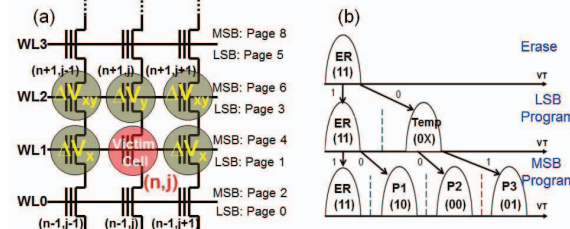
Fig. 1. (a) All-bit-line NAND flash architecture with victim cell circled in red and aggressor cells circled in grey; (b) Two-bit MLC flash programming scheme. Cell states are encoded in format (LSB, MSB)
