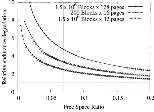
Figure 17: Degradation in performance due to wear-leveling for uniformly-distributed page writes. The vertical line marks a free percentage of 6.7%, corresponding to usage of 10^9 out of every 2^{30} bytes.
