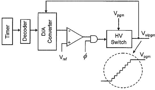
Fig. 7. Schematic of ramping circuit.
