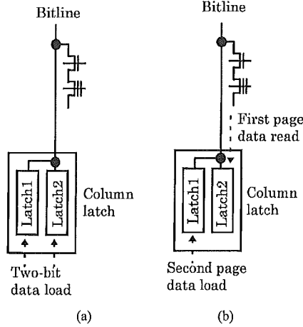
Fig. 15. Data load operation of (a) the conventional method and (b) the second page program of the proposed method.
