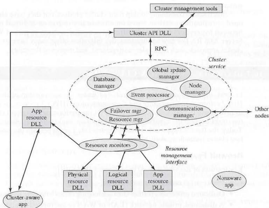
Figure 16.17 Windows Cluster Server Block Diagram
