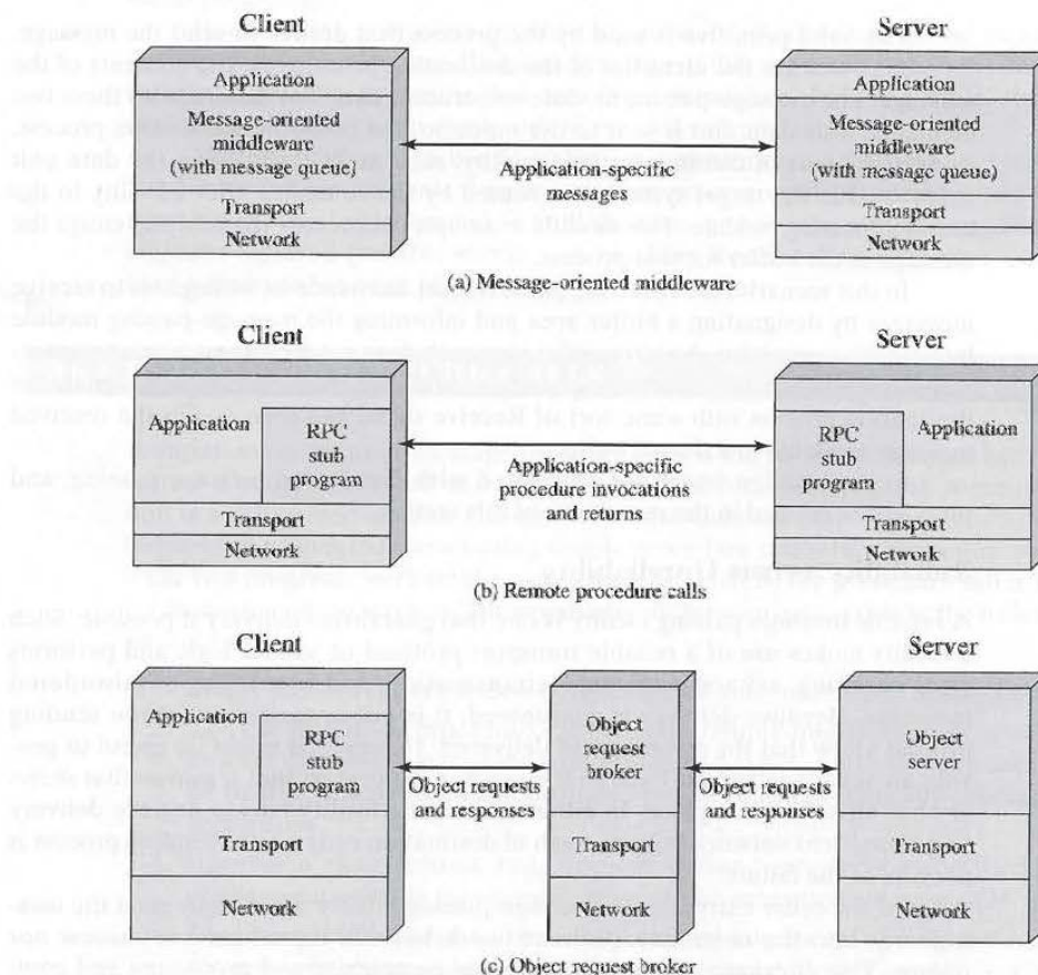
Figure 16.12 Middleware Mechanisms
