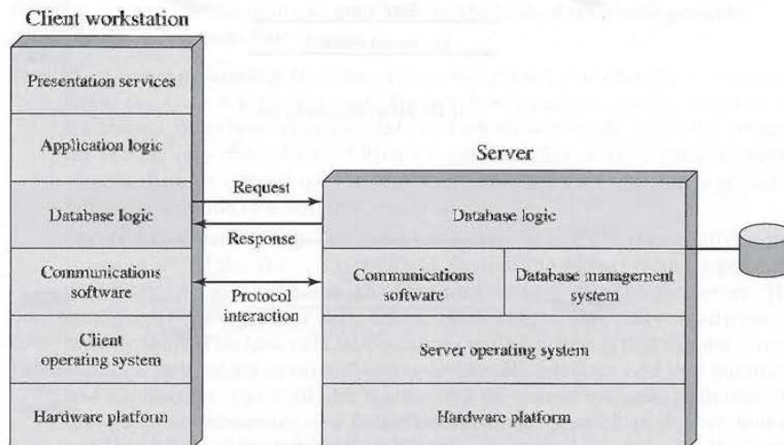
Figure 16.3 Client/Server Architecture for Database Applications
