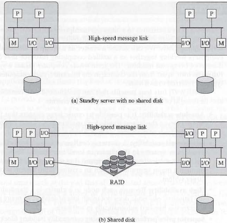
Figure 16.15 Cluster Configurations
