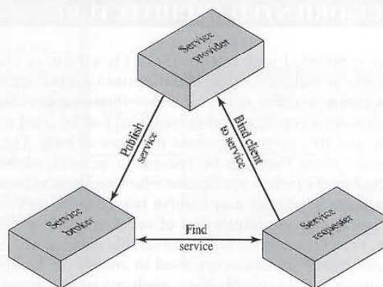
Figure 16.10 SOA Model
