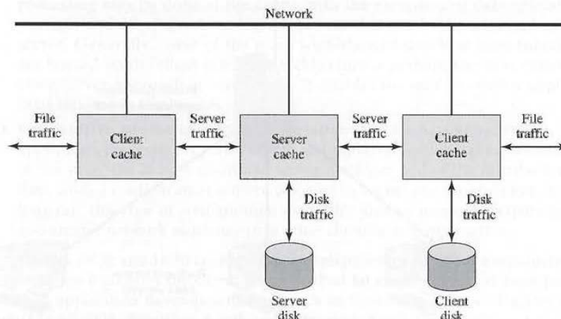
Figure 16.7 Distributed File Caching in Sprite
