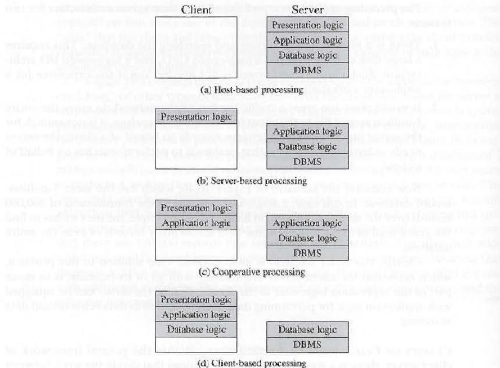
Figure 16.5 Classes of Client/Server Applications
