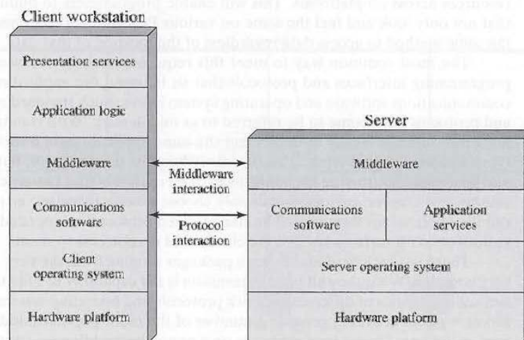
Figure 16.8 The Role of Middleware in Client/Server Architecture
