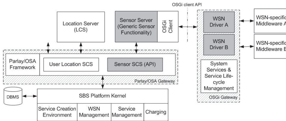
Figure 3. The distributed architecture of the overall SBS system
