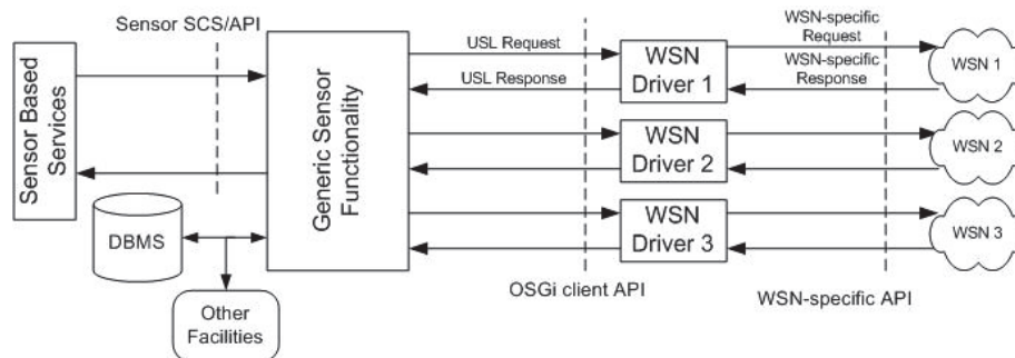
Figure 4. The proposed software architecture for SBS provisioning
