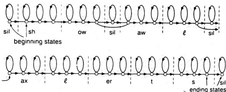
Figure 8.4 Creation of composite FSN for sentence "Show all alerts."
