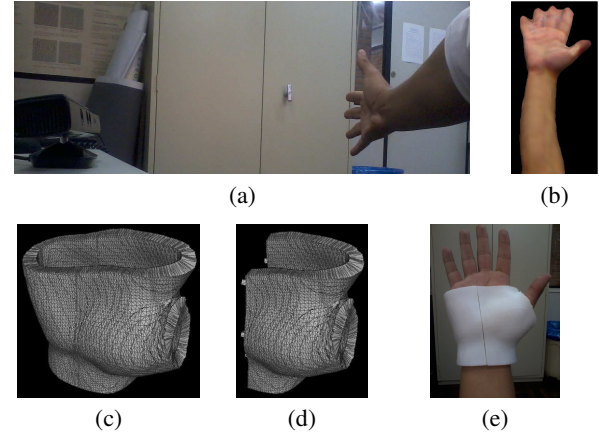
Fig. 3. Generation of an initial orthosis prototype to immobilize a wrist fracture. (a) 3D scanning, (b) reconstructed arm model adapted to anatomic shape of the user, (c) the model is cut to obtain the interest surface and then a hollow model is created to put in the wrist, (d) the mesh is segmented by one cutting plane and connectors are generated to join parts, and (e) finally, the prototype is printed in ABS and put on the wrist.
