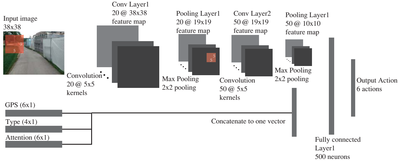
Figure 4. CNN_GPS_Recog architecture for outdoor navigation. The three subsidiary signals are concatenated into one feature vector, which is then combined with the high level feature vector generated by two rounds of convolution and max-pooling over the input image. A two layer fully connected neural network is then deployed on top of the feature vector to generate the final output action. This architecture can be trained using stochastic gradient descent (SGD) and error-back propagation. We compare the performance of this architecture with our Developmental Network in Sec.4.1. The CNN_GPS network shares the same architecture as the CNN_GPS_Recog in convolution and pooling parameters, but there are no available type and attention information for CNN_GPS during training.
