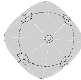
Figure 16: Curvature extrema edges detected on rounded octahedron.
