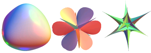
Figure 6: Left: a rounded octahedron. Middle and right: the sheets of the focal surface of the octahedron.
