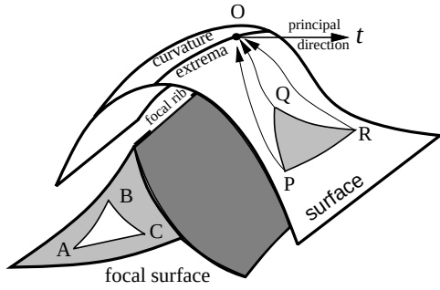
Figure 4: Surface and Focal Surface.
