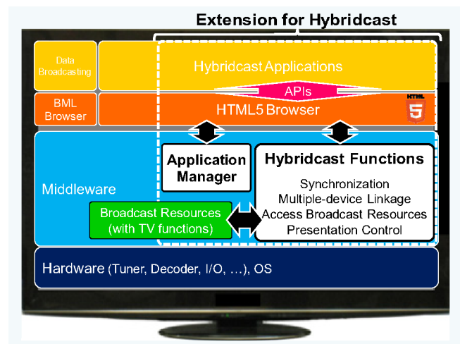
Figure 9. Architecture of a Hybridcast receiver
