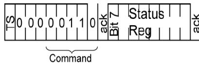
Figure 7 Status Register Write
