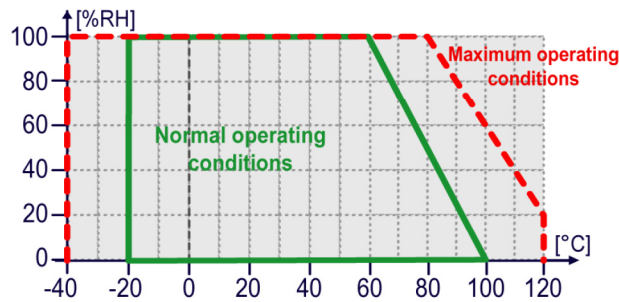
Figure 11 Recommended operating conditions
