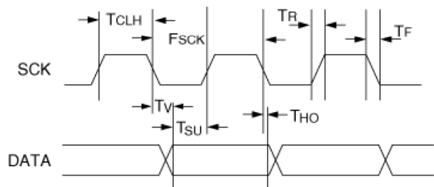
Figure 9 Timing Diagram
