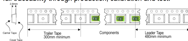
Figure 12 Tape configuration and unit orientation
