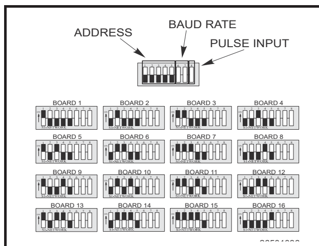
Figure 4-10 - Network Address Settings for Dip Switch S1 or S3 on I/O Boards
