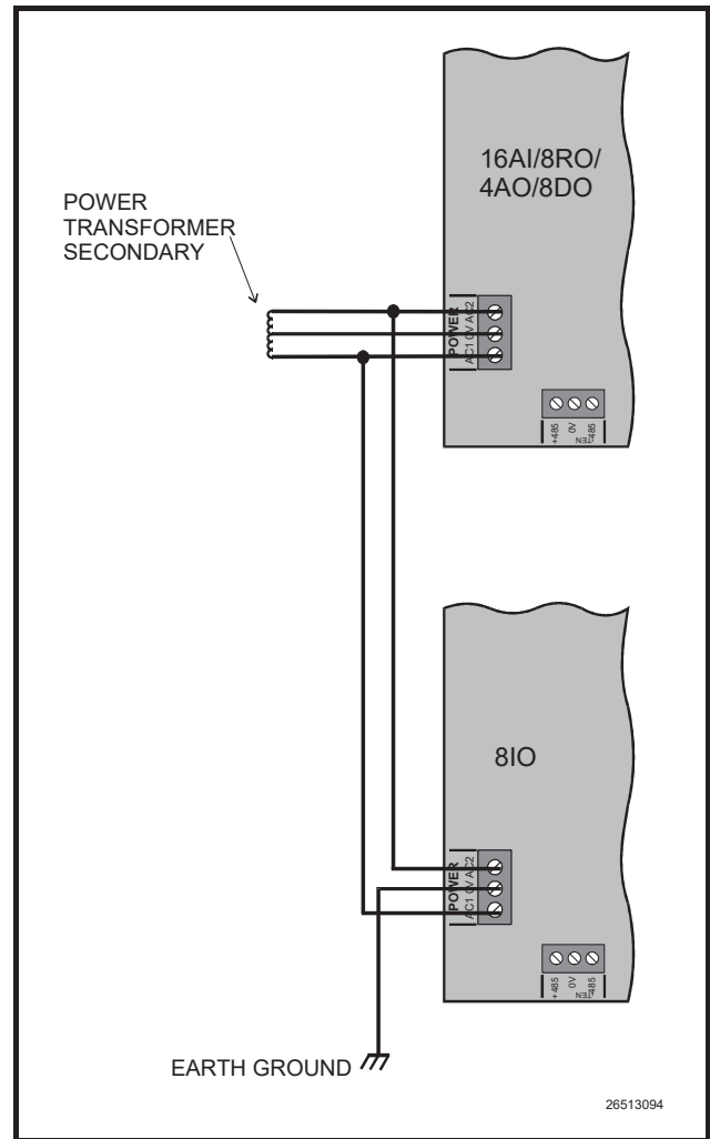
Figure 5-11 -8IO Board Wired in Combination with A or Multiple 16AI, 8RO, 4AO, 8DO
