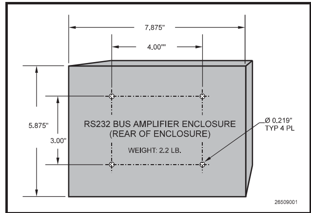
Figure 3-11 - RS232 Bus Amplifier Mounting Dimensions
