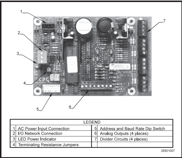
Figure 2-6 - 4AO Analog Output Board
