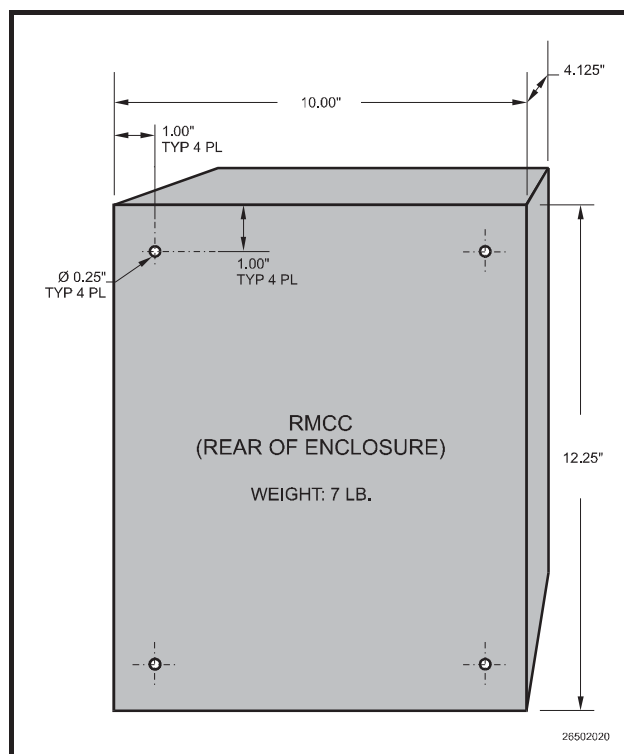
Figure 3-1 - RMCC Mounting Dimensions
