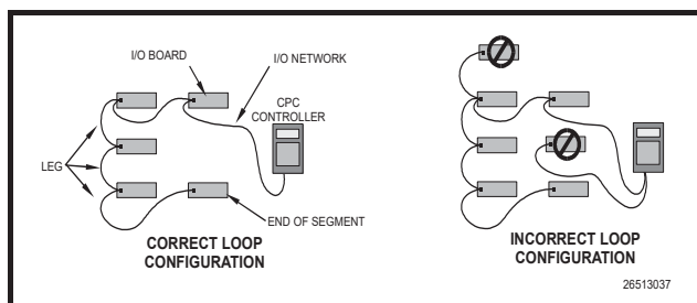
Figure 4-5 - Correct and Incorrect Loop Configurations
