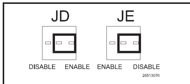
Figure 5-5 - Fincor Inverter Dip Switch Settings
