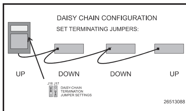
Figure 4-7-Terminating Jumpers for a "Daisy Chain" Configuration
