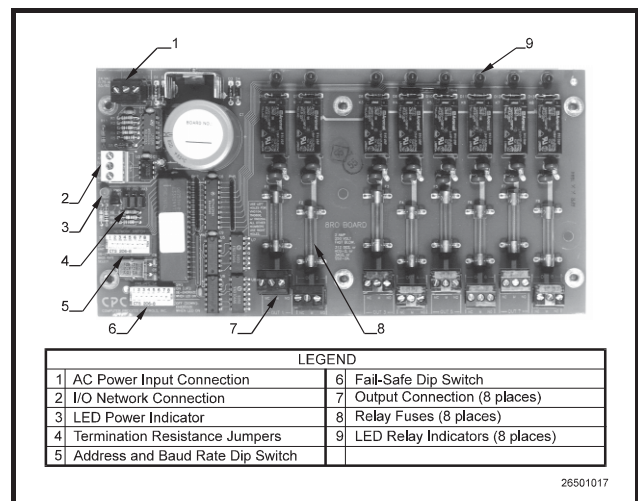
Figure 2-5 - 8RO-FC Relay Output Board with Form C Contacts
