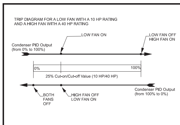
Figure 9-5 - Diagram of Two-Speed Condenser Operation
