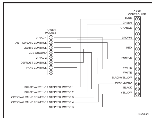
Figure 7-5 - Output Cable Harness With Quick Connects (335-3158) Schematic Diagram
