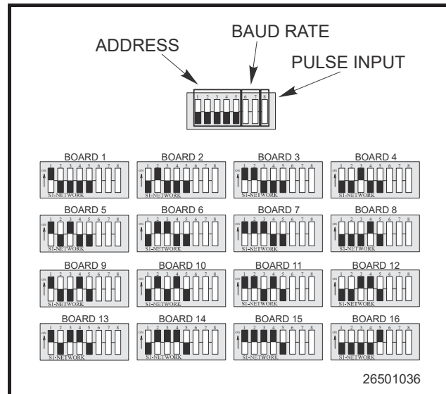
Figure 5-13 - Network Address Settings for Dip Switch S1 or S3 on I/O Boards
