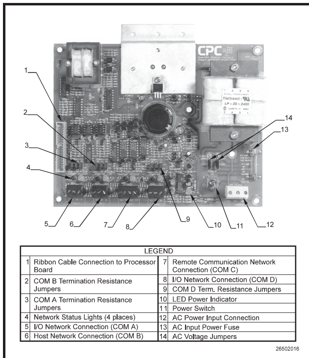
Figure 2-2 - Power Interface Board
