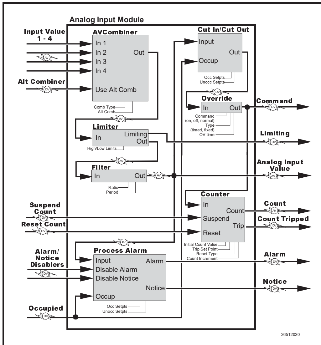
Figure 9-9 - Analog Input Module
