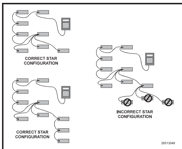
Figure 4-6 - Correct and Incorrect Star Configurations
