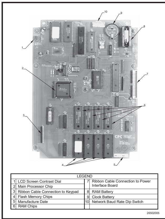
Figure 2-1 - REFLECS Processor Board
