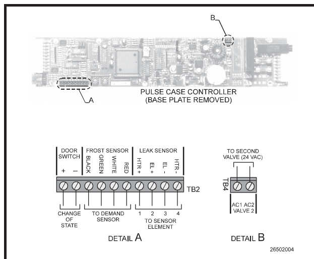
Figure 7-2 - Case Controller Optional Inputs and Outputs Wiring
