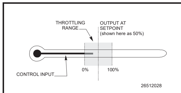
Figure 9-1 - PID Proportional Mode Diagram
