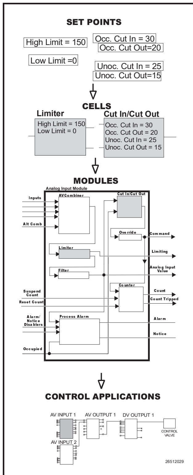
Figure 9-8 - Relationship Between Set Points, Cells, and Modules
