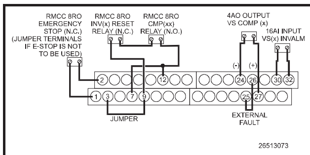
Figure 5-4 - Fincor Inverter Control Wiring
