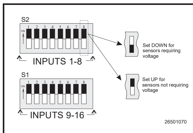
Figure 5-16 - Input Type Switches (S1 and S2)
