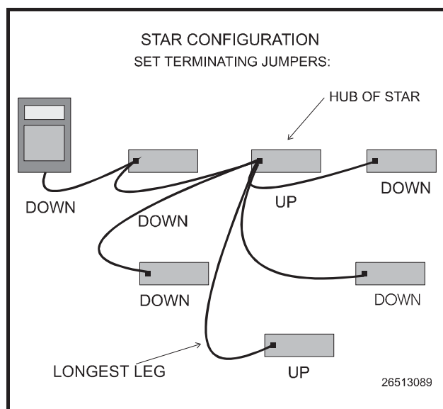
Figure 4-8-Jumper Settings for Star Network
