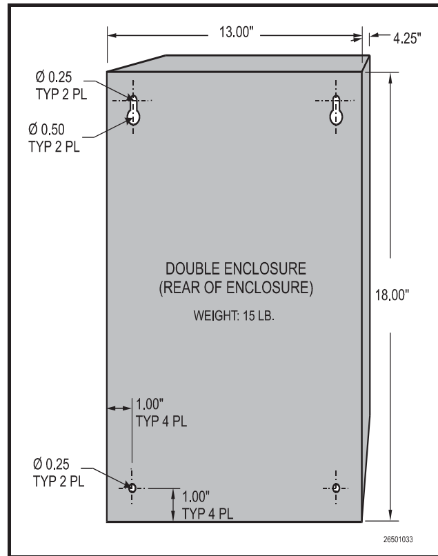
Figure 3-3 - Double Enclosure Mounting Dimensions
