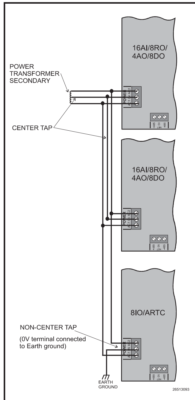
Figure 5-9-Wiring for Three 16AIs, 8ROs, 4AOs, or 8DOs or Any Combination of
