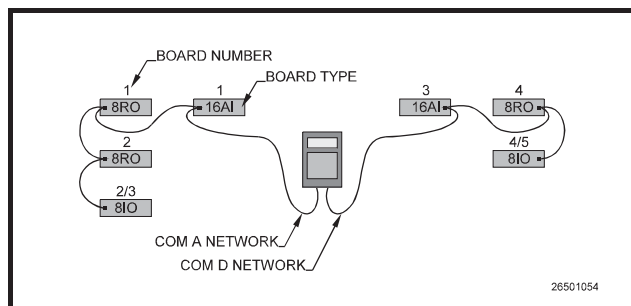
Figure 4-9 - Network Device Numbering
