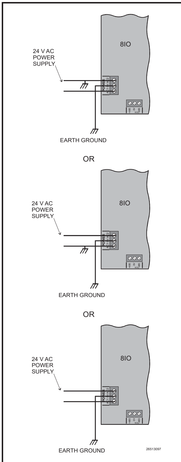
Figure 5-12 -One 8IO Wired to a 24 V AC Line with a Ground on Either Side
