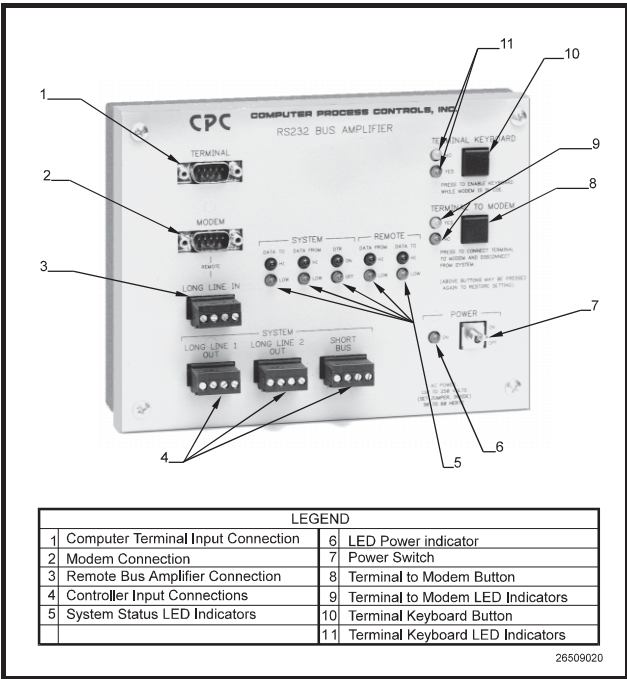
Figure 2-11 - RS232 Bus Amplifier
