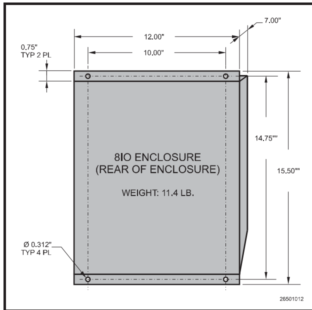
Figure 3-4 - Weather Resistant Enclosure
