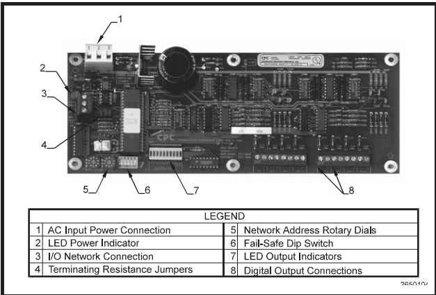
Figure 2-7 - 8DO Digital Output Board
