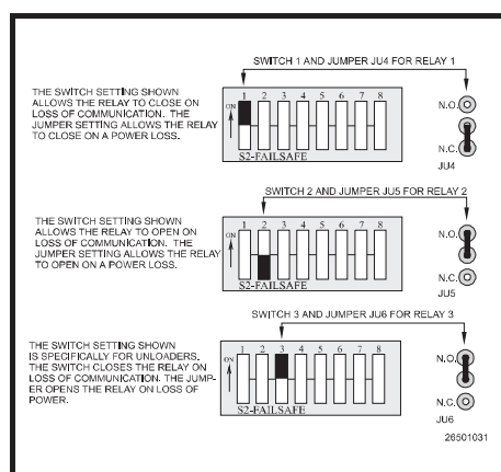
Figure 5-14 - 8RO Board Fail-Safe Dip Switch and Jumper Settings
