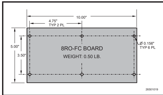
Figure 3-7 - 8RO-FC Mounting Dimensions
