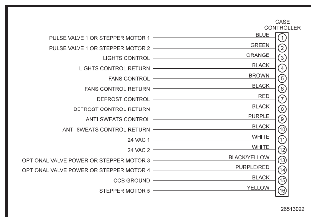
Figure 7-4 - Output Cable Harness Without Quick Connects (335-3156) Schematic Diagram
