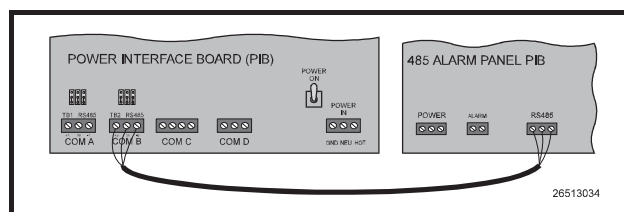
Figure 5-2 - COM B Network Connections
