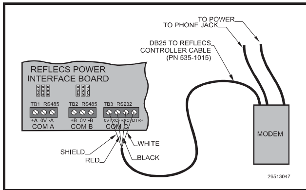
Figure 5-3 - COM C Network Connection
