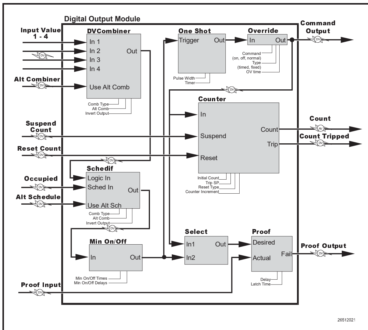
Figure 9-11 - Digital Output Module
