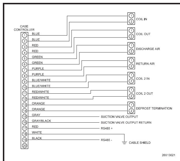
Figure 7-3 - Input Cable Harness (335-3151) Schematic Diagram
