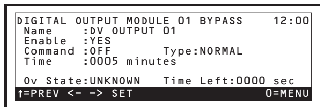
Figure 9-12 - Digital Output Module Bypass Screen
