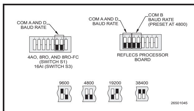
Figure 5-15 - Baud Rate Dip Switch Settings
