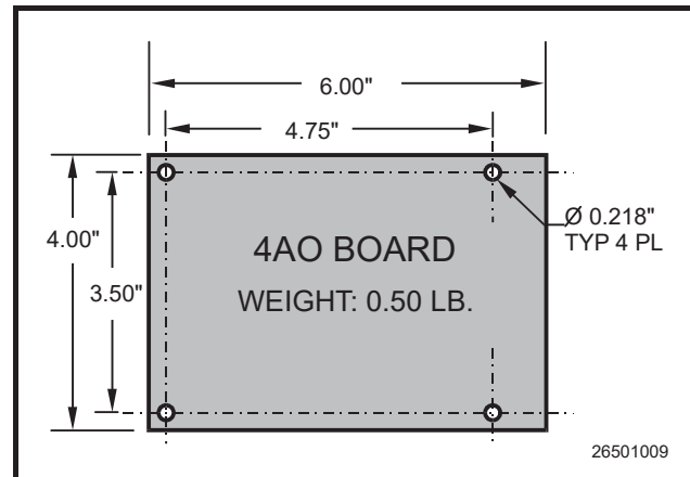
Figure 3-9 - 4AO Mounting Dimensions
