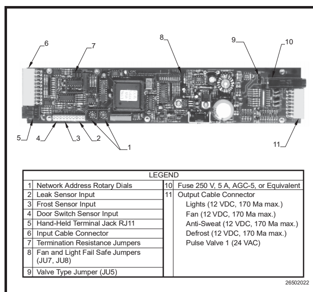
Figure 6-2 - Stepper EEV Case Controller
