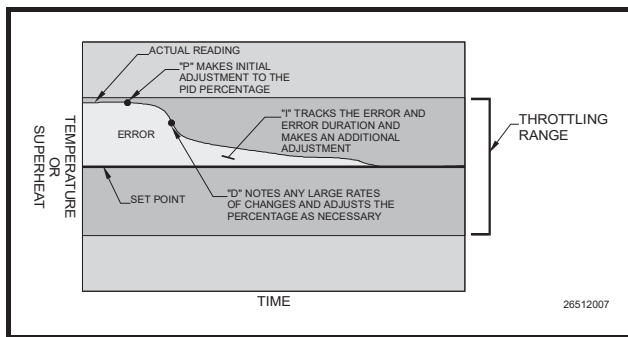
Figure 9-2 - Typical PID Control
