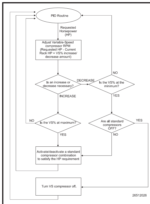
Figure 9-3 - VS Compressor Control Flowchart
