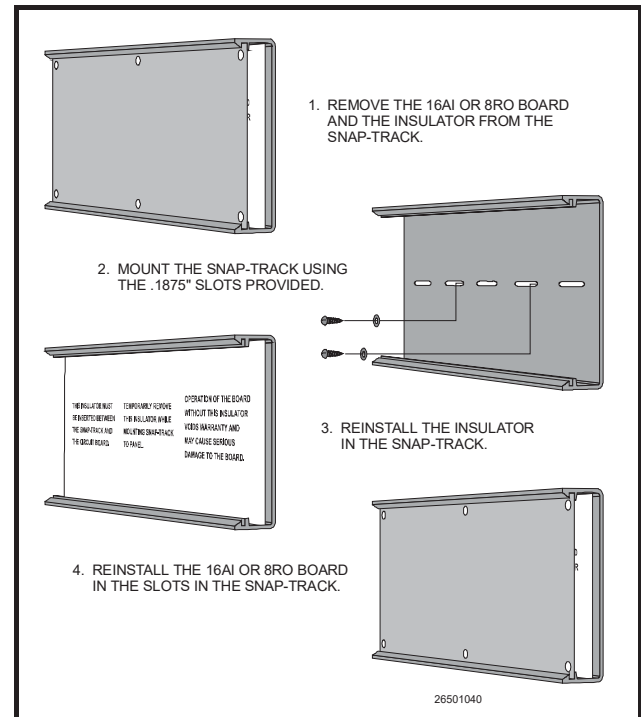
Figure 3-5 - 4AO, 8RO, or 16AI Snap-Track Installation
