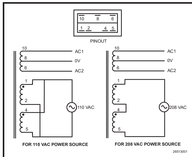
Figure 5-7 - Wiring for 640-0043, Three Board, and 640-0045, Six Board Transformer
