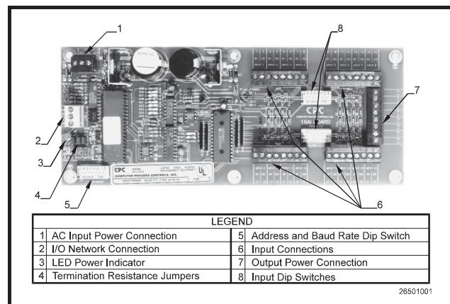
Figure 2-3 - 16AI Analog Input Board
