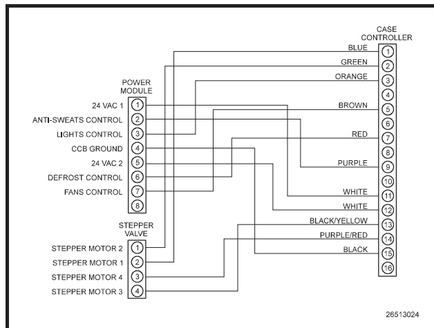
Figure 7-6 - Sporlan Stepper Valve Output Cable Harness (335-3159) Schematic Diagram
