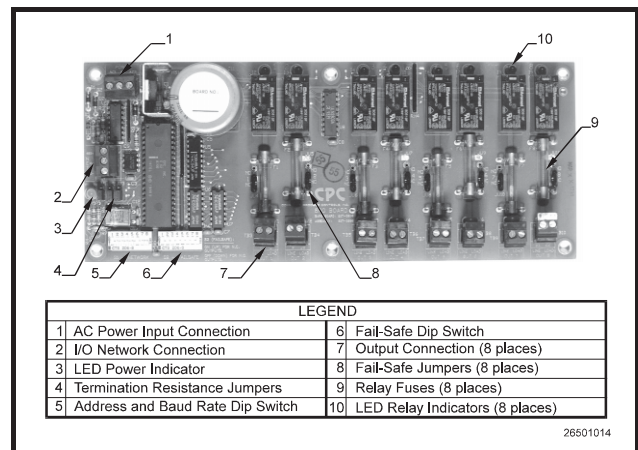
Figure 2-4 - 8RO Relay Output Board
