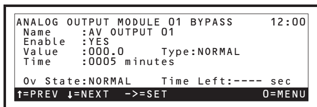
Figure 9-15 - Analog Output Module Bypass Screen
