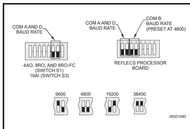
Figure 4-11 - Baud Rate Dip Switch Settings
