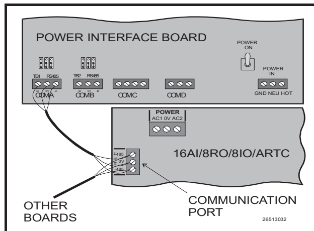
Figure 5-1 - COM A Network Connections
