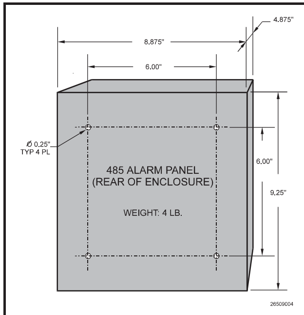
Figure 3-10 - 485 Alarm Panel Mounting Dimensions
