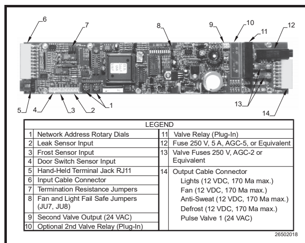
Figure 6-1 - Pulse EEV Case Controller
