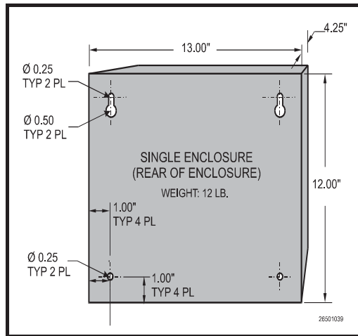
Figure 3-2 - Single Enclosure Mounting Dimensions
