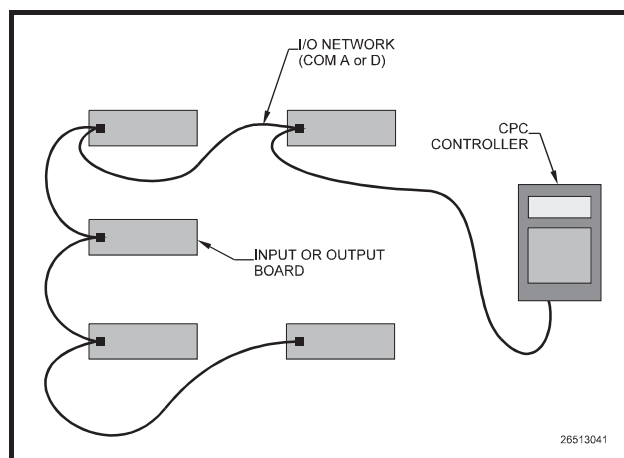
Figure 4-1 - Network Loop Wiring Configurations
