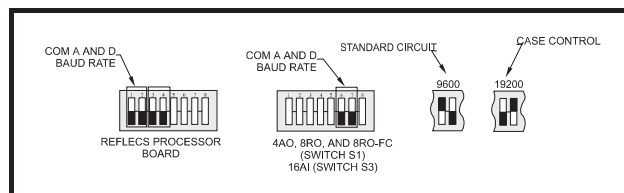
Figure 4-12-Baud Rate Dip Switch Settings
