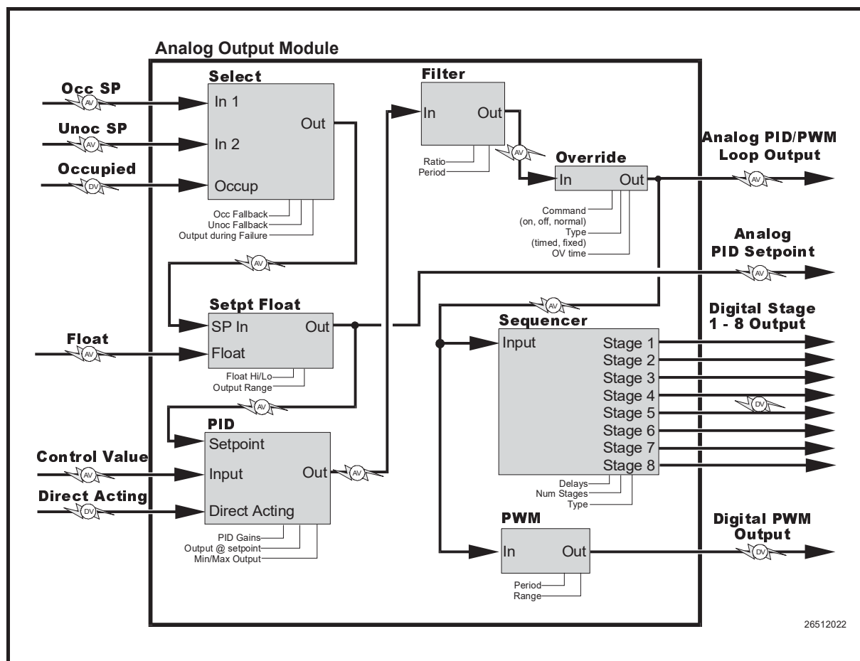
Figure 9-13 - Analog Output Module
