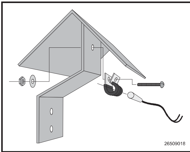
Figure 3-12 - Outside Temperature Sensor with Cover and Clamp
