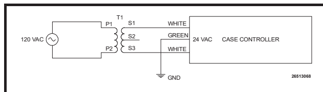
Figure 7-1 - Case Controller to Transformer Wiring
