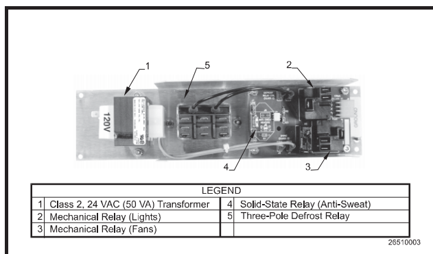
Figure 6-4 - Case Controller Power Module Without Fuse Protection
