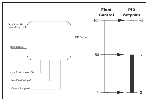
Figure 9-14 - Example of a Setpt Float cell
