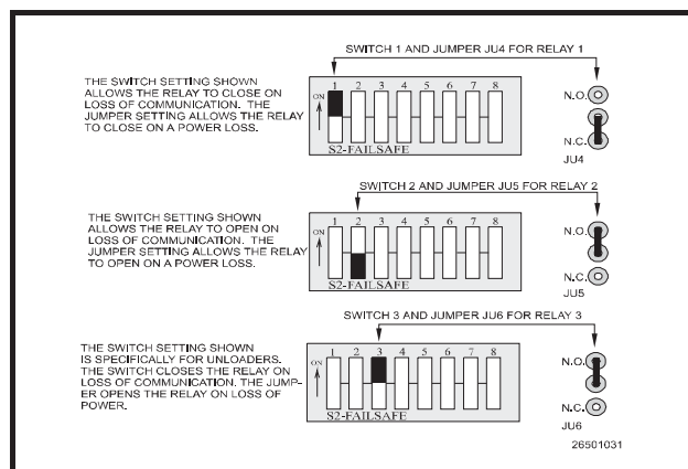
Figure 4-13 - 8RO Board Fail-Safe Dip Switch and Jumper Settings
