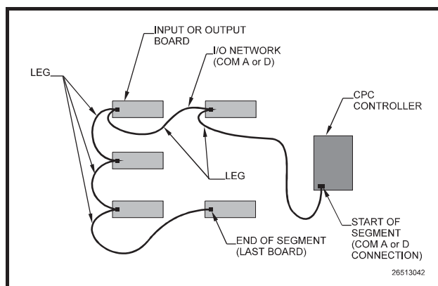
Figure 4-4 - Relationship Between Legs and a Segment
