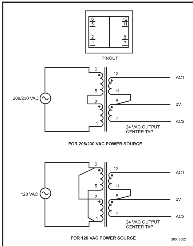
Figure 5-8 - Wiring for 640-0048, Ten Board Transformer
