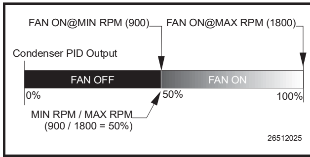
Figure 9-6 - Diagram of Variable-Speed Condenser Operation
