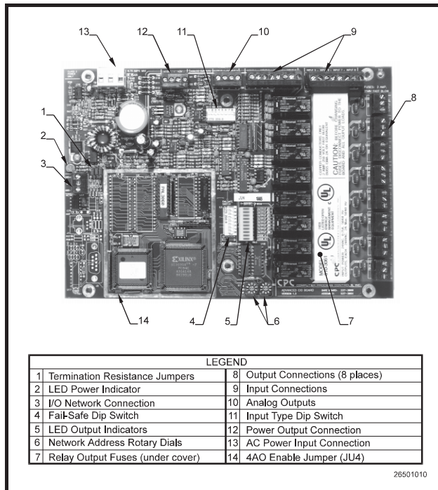
Figure 2-8 - 8IO Combination Input/Output Communication Board
