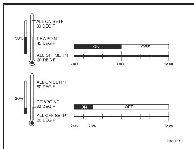
Figure 9-7 - Illustration of Anti-Sweat Control
