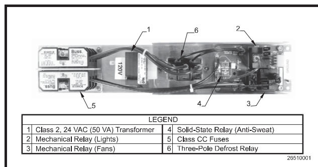
Figure 6-3 - Case Controller Power Module
