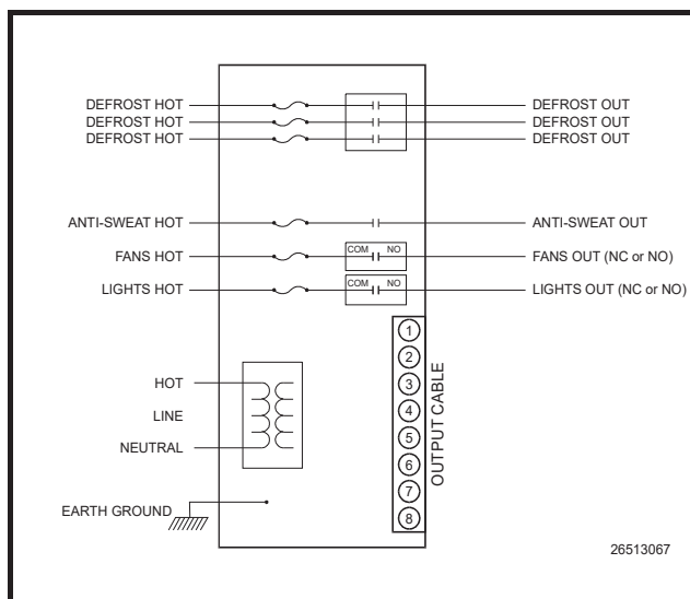
Figure 7-7 - Case Controller and Defrost Power Module Wiring Schematic
