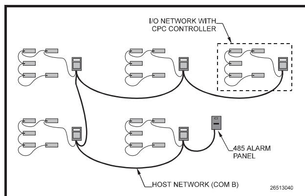
Figure 4-2 - RS485 Host Communication Network (COM B)
