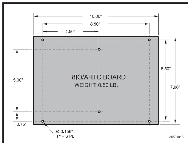
Figure 3-8 - 8IO/ARTC Mounting Dimensions
