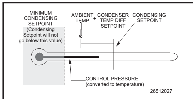
Figure 9-4 - Temperature Differential Strategy
