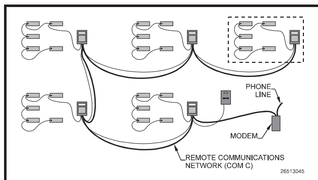
Figure 4-3 - RS232 Remote Communication Network (COM C)
