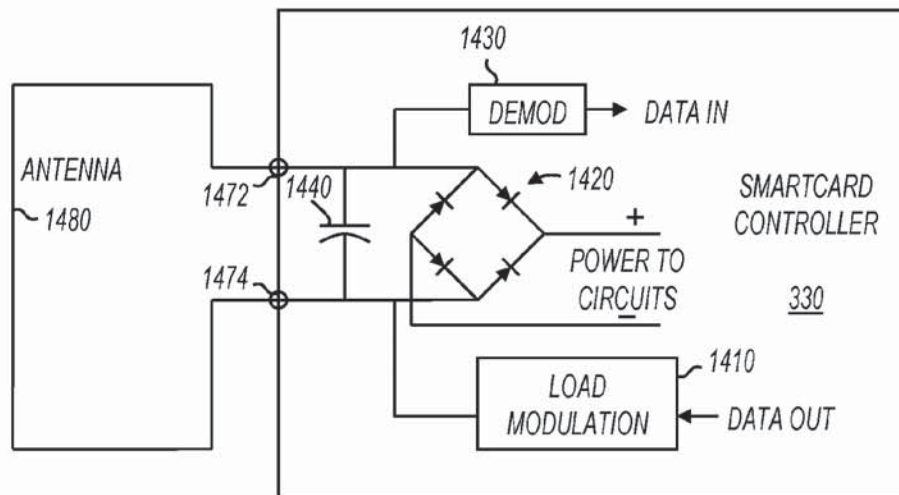
FIG. 14 (PRIOR ART)
