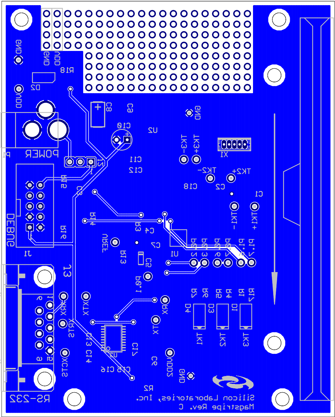
Figure 1. Bottom Layer (Mirrored, 3.9375" x 3.375")
