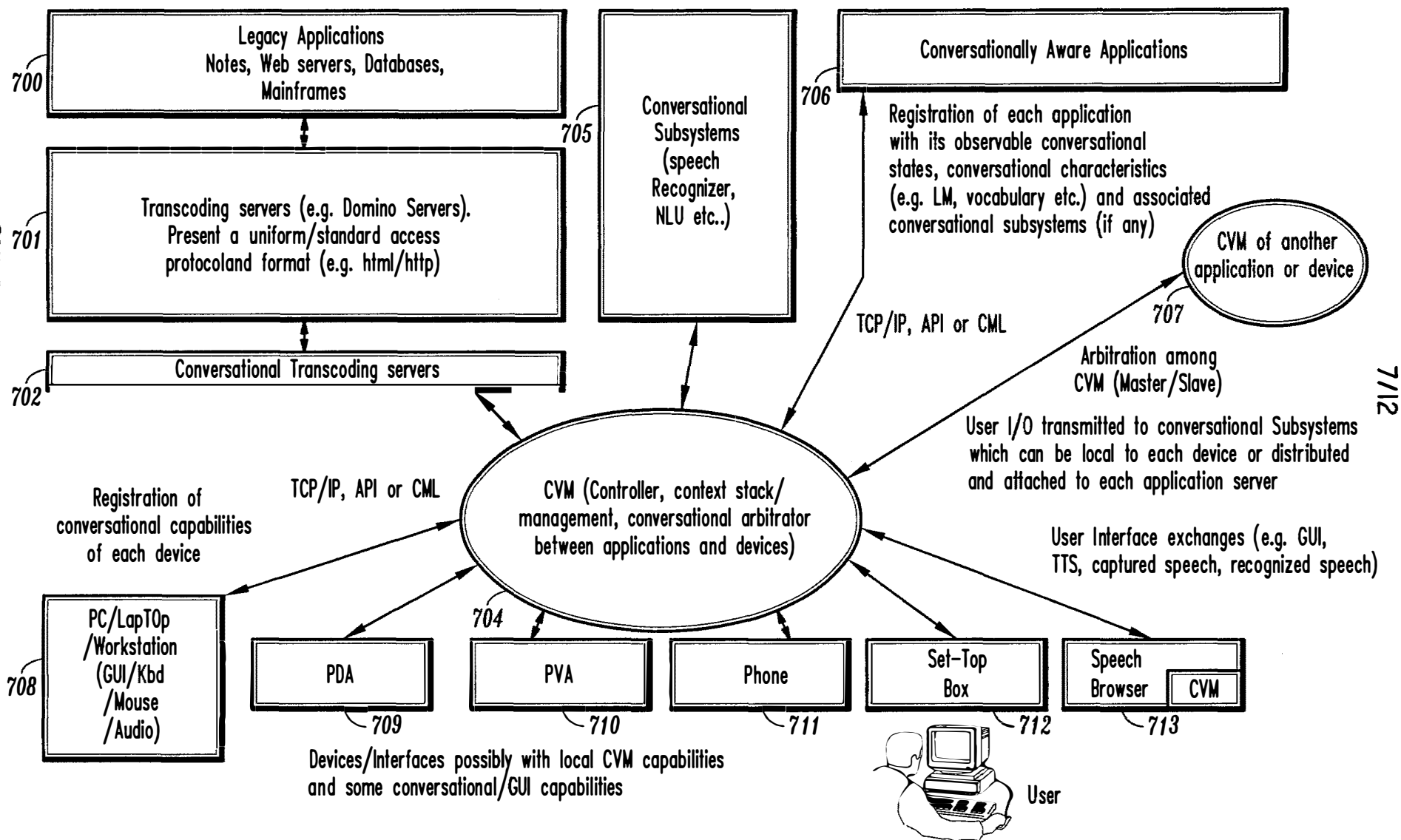
FIG. 7 Architecture for a Distributed CVM
