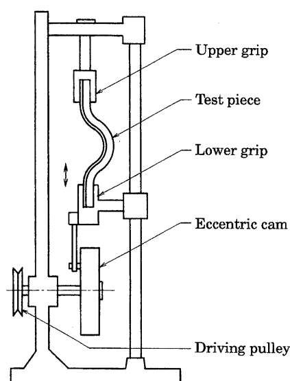
Annex 1 Fig. 4 Compression/bending tester of De Mattia method (method B)
