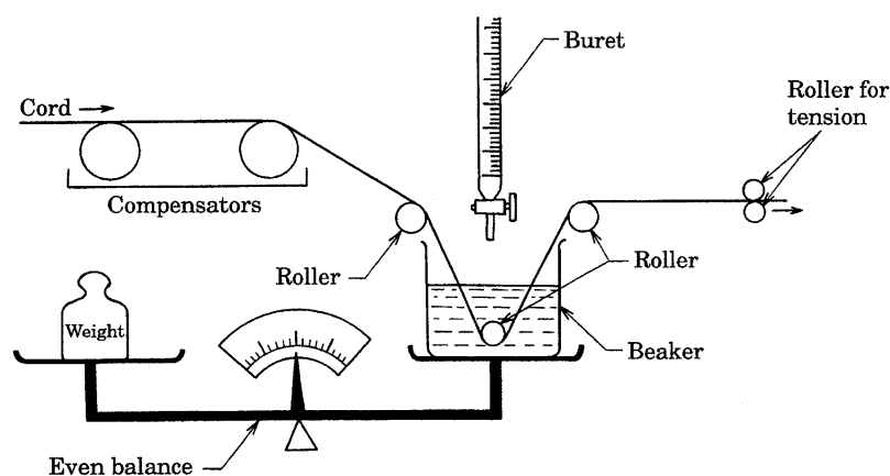
Fig. 3 Measuring apparatus for water absorption
