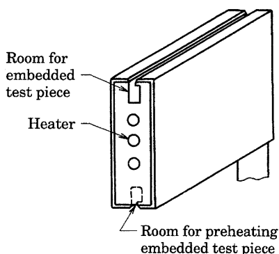
Annex 1 Fig. 13 Fixing device for embedded test piece
