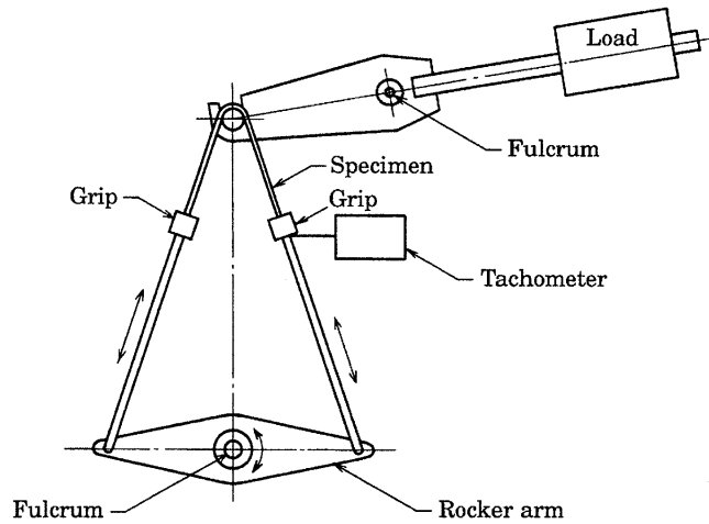
Annex 1 Fig. 1 Compression/bending tester of Firestone method (method A)
