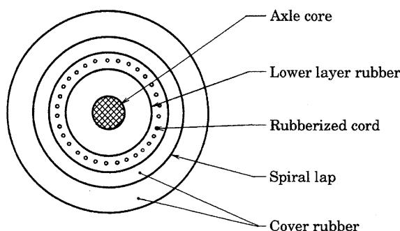
Annex 1 Fig. 7 Construction of rubber tube-type test piece
