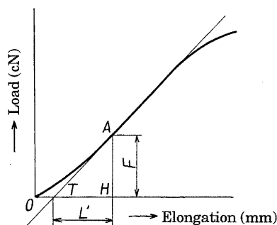
Fig. 2 Load-elongation curve
