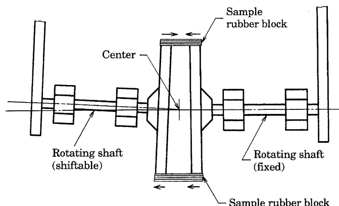
Annex 1 Fig. 8 Disc-type fatiguing strength tester
