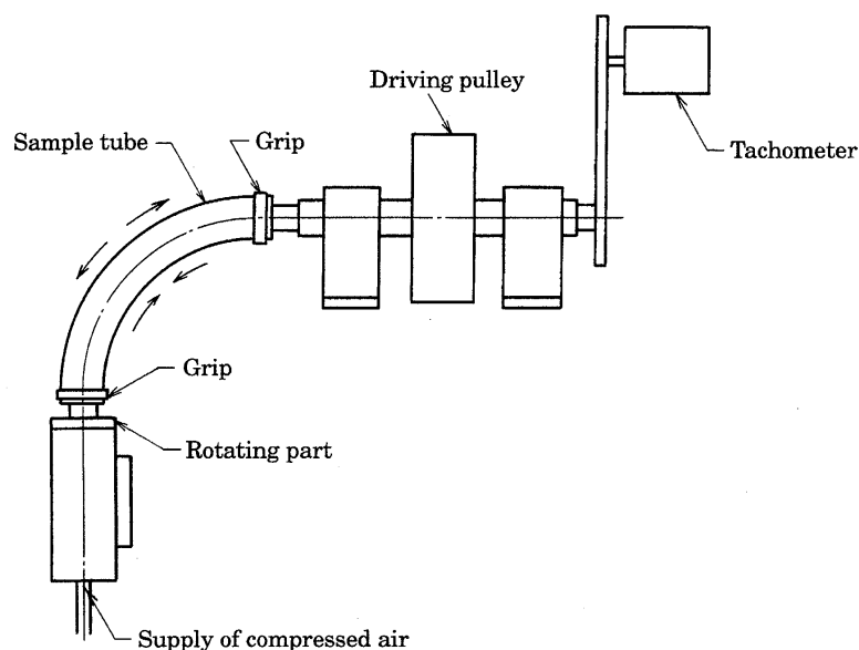
Annex 1 Fig. 6 Extension/compression fatigue tester of Goodyear method
