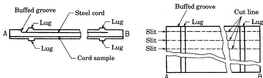
Annex 1 Fig. 3 Buffed groove
