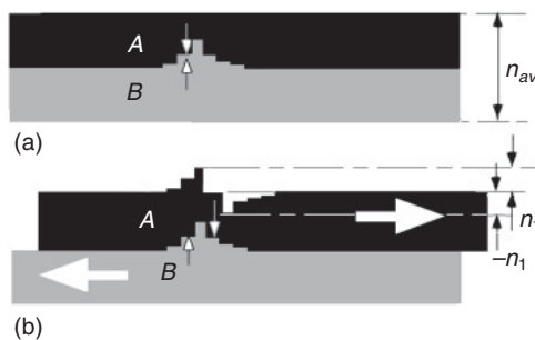
Fig. 3.21 Longitudinal fiber migration and strand evenness
