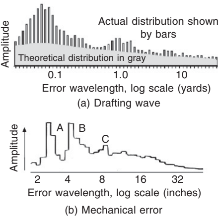
Fig. 3.18 Actual and theoretical variance distributions in a drawframe sliver
