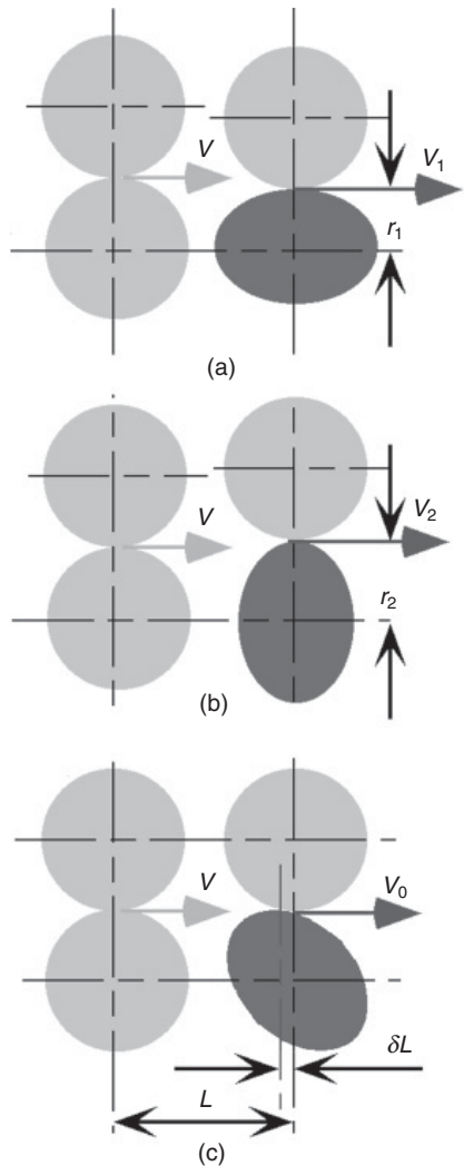
Fig. 3.14 Deformed rolls
