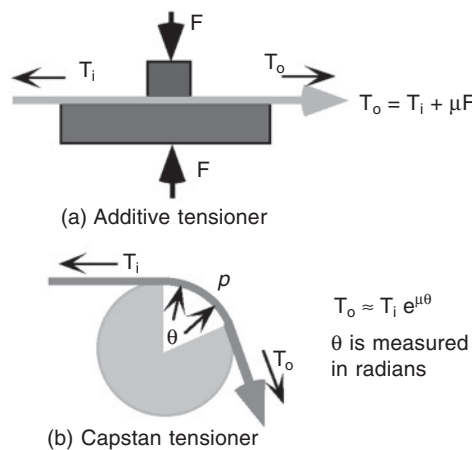
Fig. 3.12 Tension controllers
