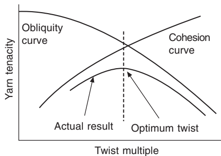
Fig. 3.2 Effect of twist on yarn strength
