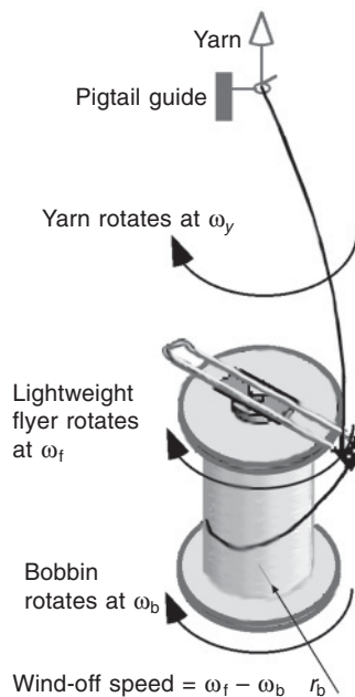
Fig. 3.7 Up-twist (up-twist is used to wind yarn from a package)
