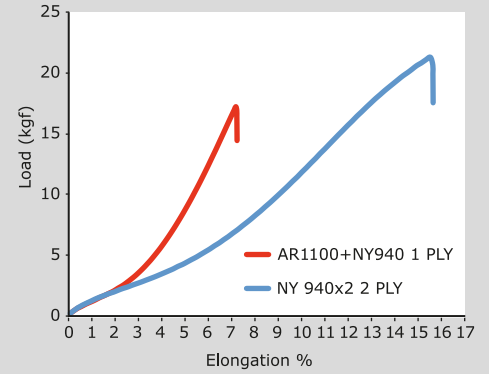
Force & Elongation @ 70C
