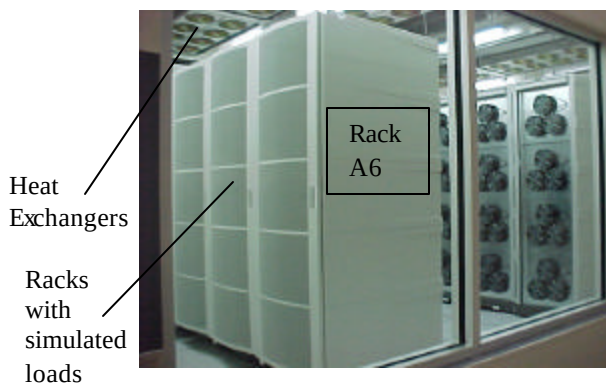
Figure 3. Prototype Data Center
