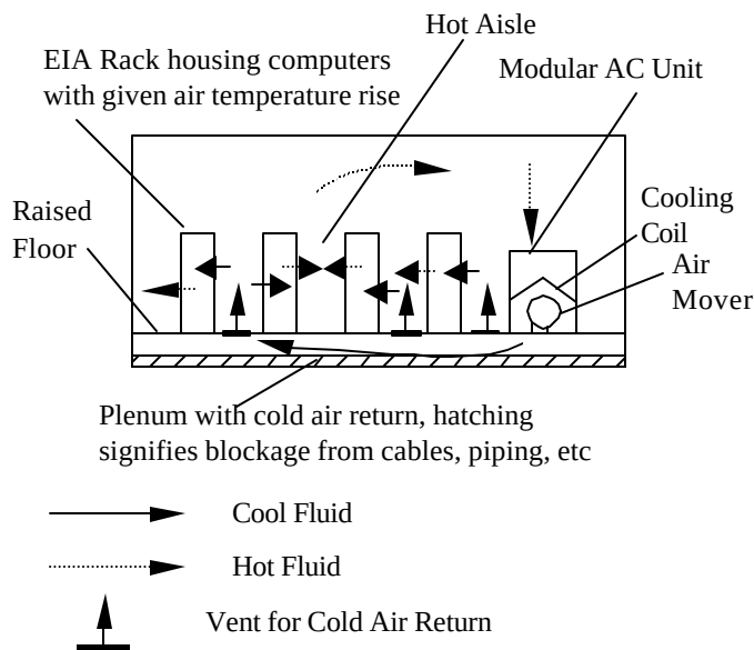
Figure 1. Typical Data Center Configuration
