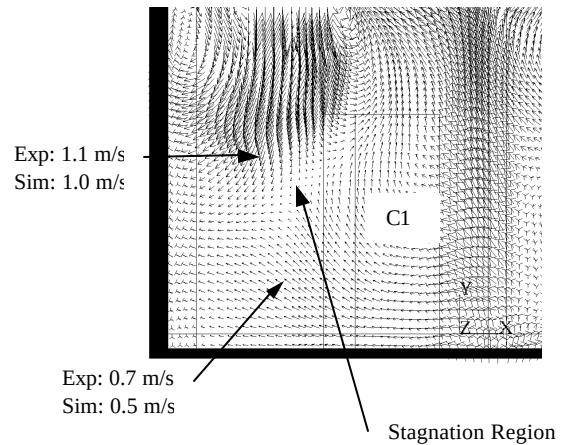
Figure 18. Velocity map at Z = 4.9 m near rack C1.
