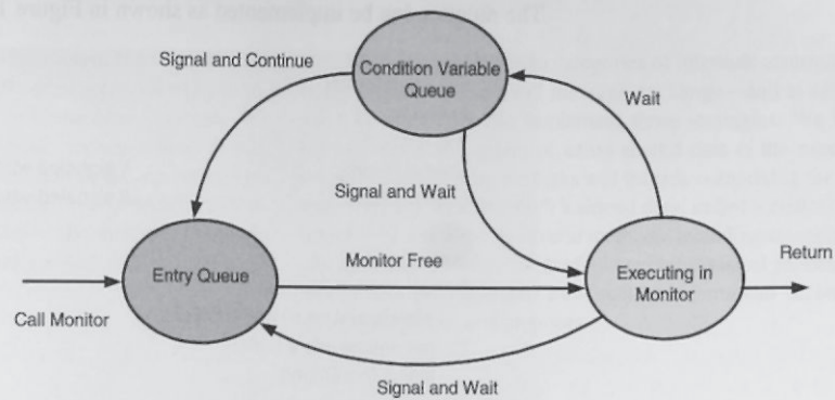
Figure 12.45 A State Diagram Model for a Monitor
