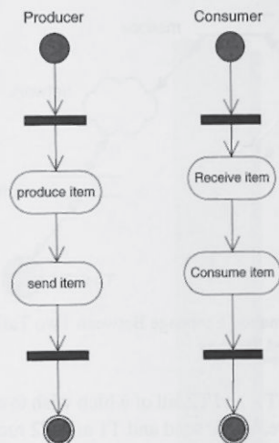
Figure 12.18 Activity Diagram Illustrating a Producer-Consumer Exchange
