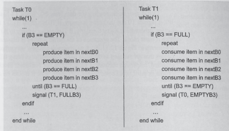
Figure 12.13 Information Sharing Between Tasks Executing at Different Speeds
