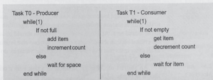
Figure 12.28 Pseudo-Code Modeling a Producer–Consumer Information Exchange
