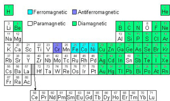
Figure E. Diagram of a periodic table showing elements coloured according to the type of magnetism they show at room temperature.
