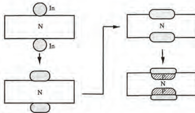
Figure 1-6 Alloy junction technology of the 1950s.
