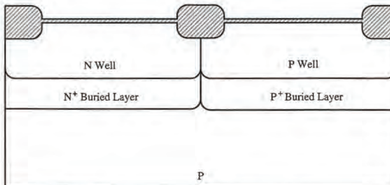
Figure 2-21 Process option incorporating buried and epitaxial layers.
