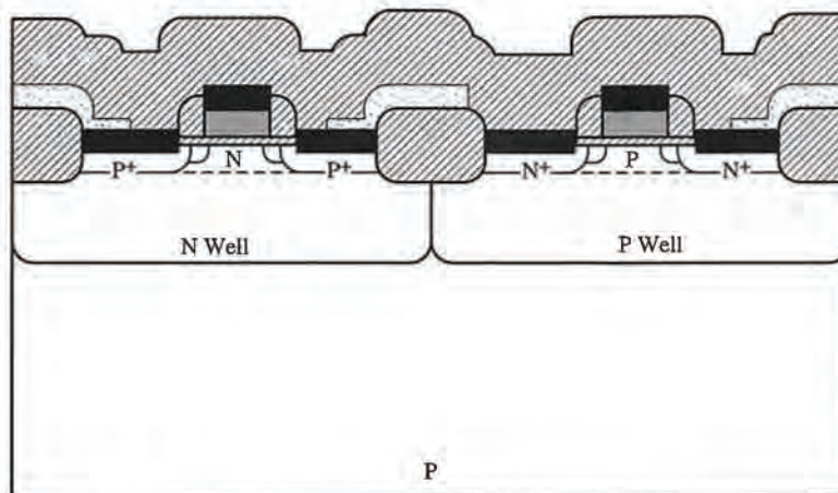
Figure 2-38 After stripping the photoresist, a conformal \text{SiO}_2 layer is deposited by LPCVD.
