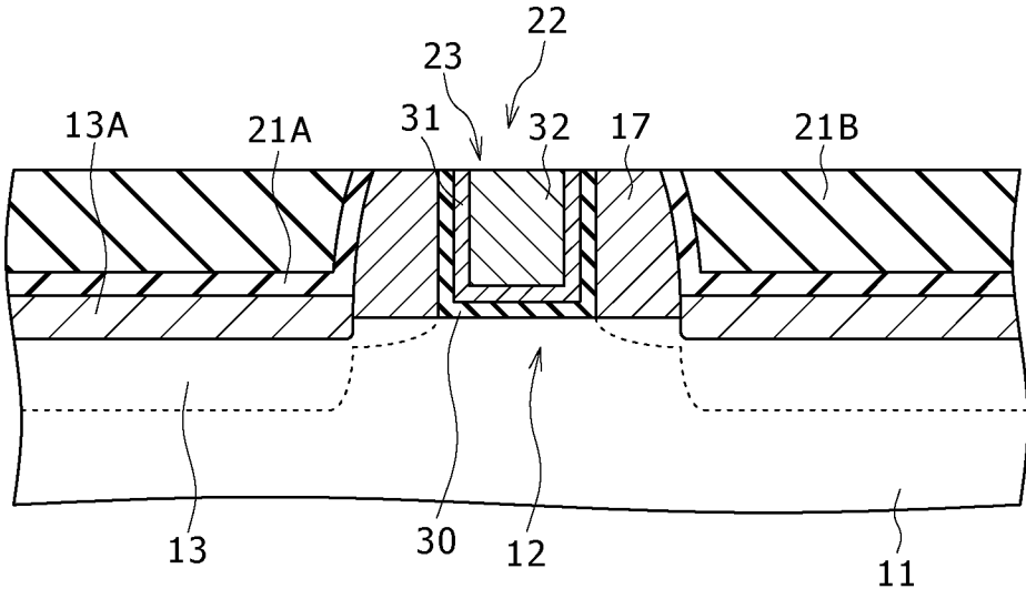
FIG. 2F [PROCESS-210]
