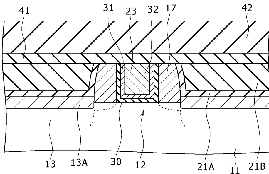
FIG. 4A [PROCESS-410]
