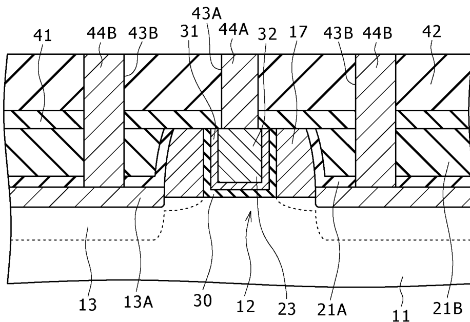
FIG. 4B [PROCESS-420]
