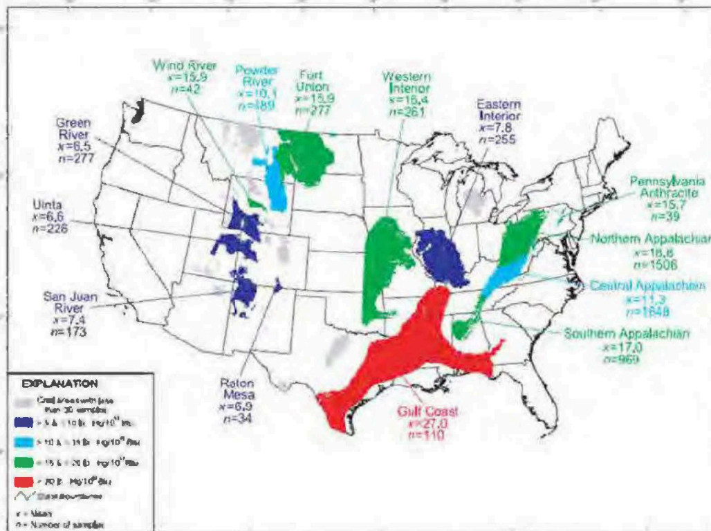
Figure 3. Mercury input loadings (in pounds of mercury per 10 9 British thermal units (lb Hg/10 9 Btu)) of in-ground coal for selected U.S. coal-producing regions.
