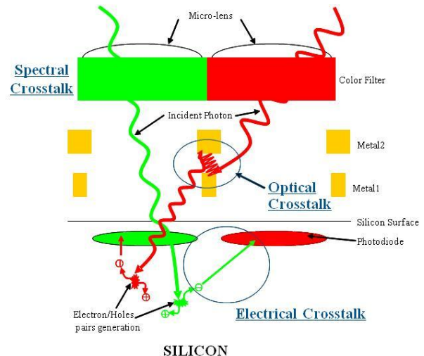
Fig. 1. Illustration for mechanism of electrical and optical crosstalk in image sensor
