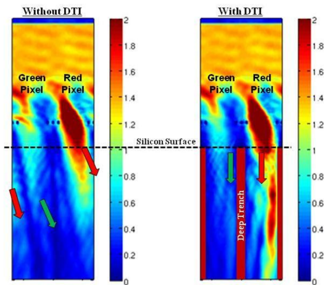
Fig. 7. Off-axis optical Simulation @633nm of 1.4 \mu pixel in FSI : Comparison between pixel with isolation by implantation and isolation by Deep Trench
