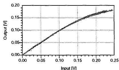
Figure 4: Simulated AM-AM Characteristic of SHF-0189 when f_s 5.3 MHz (67% of output signal is overlapped).
