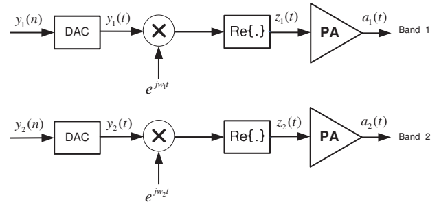
Fig. 1. Block diagram of multiple radio system.
