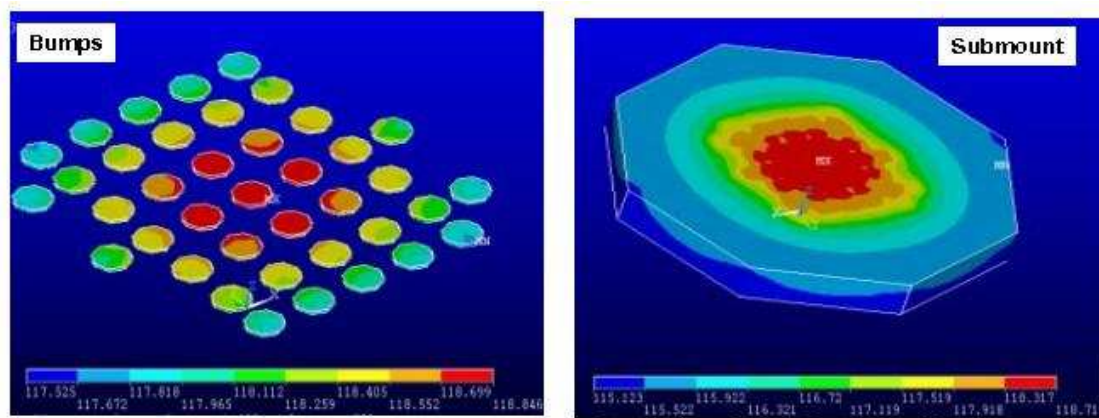
Figure 9. Temperature distribution in the bumps and submount for Sapphire chip package
