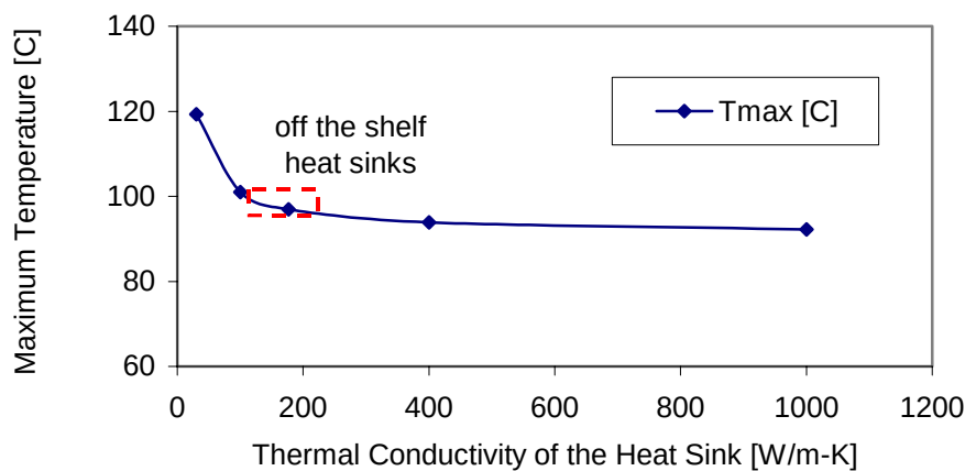
Figure 16. Variation heat sink performance with the material for 3" height fins
