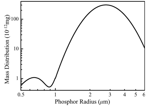
Fig. 6. Mass distribution curve of unit YAG:Ce phosphor.
