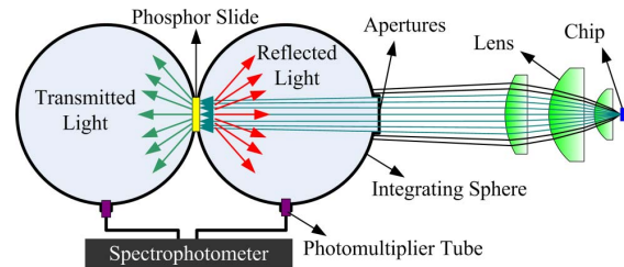
Fig. 1. (Color online) Measurement platform of YAG:Ce phosphor.
