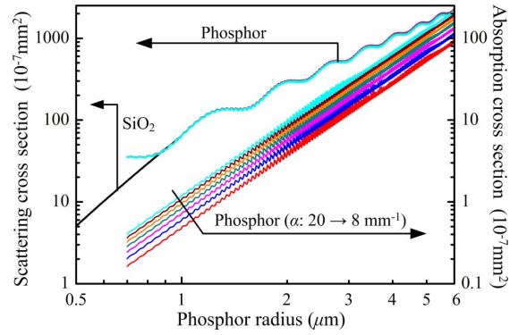
Fig. 7. (Color online) Absorption and scattering cross sections of YAG:Ce phosphor for blue light by Mie theoretical calculation.
