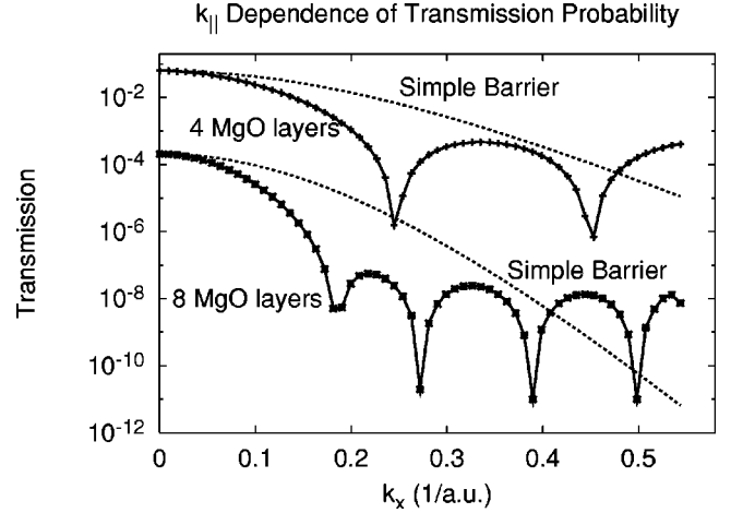
FIG. 9. Majority transmission probability as a function of k_{\parallel} for k_y = 0 for 4 and 8 layers of MgO. The curves end before the zone boundary is reached because there are no states for k_x > 0.55 (a.u.) -1 . Smooth curves show the expected behavior of the transmission probability from Eq. (9).
