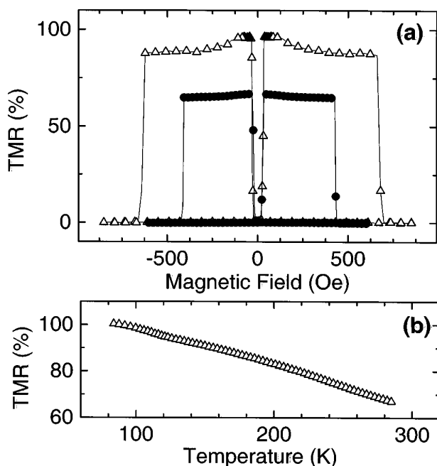
FIG. 1. (a) TMR of a 65 \times 95 \mu\text{m}^2 large MgO (100)/Fe/MgO–2.5 nm/Fe/Co/Au junction at 80 K ( \Delta ) and 293 K ( \bullet ). The measurements are performed along the easy axis, the junction being biased at 10 mV. (b) Variation of TMR at 10 mV with temperature.
