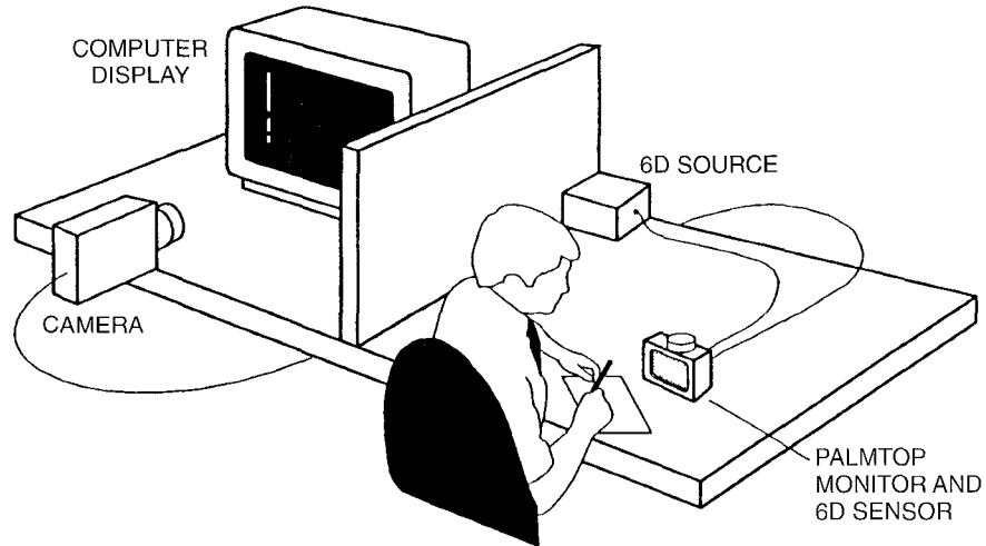
Fig. 4. Configuration of the Chameleon prototype.
