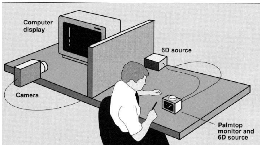
Figure 2. Configuration of Chameleon prototype
